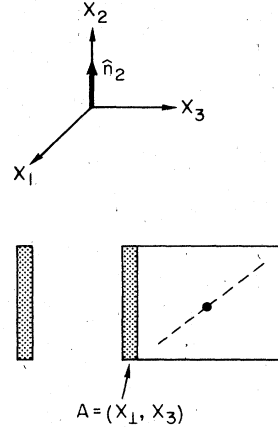
FIG. 23. \sigma_3 on a dual link is defined as a product of \sigma_1 's on the solid links.
