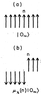
FIG. 10. A kink applied at site n flips all the spins from -\infty up to site n .
