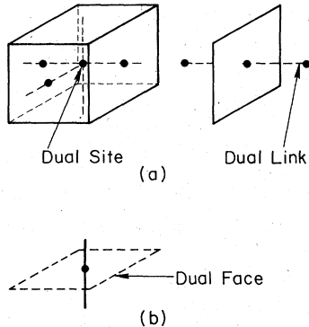
FIG. 22. The dual lattice.
