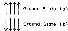
FIG. 9. The ground state of the quantum-mechanical Ising model in a transverse field at large values of \lambda is doubly degenerate.
