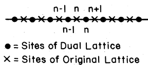
FIG. 8. Dual lattices in one dimension.
