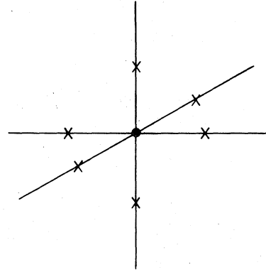
FIG. 15. In 3+1 dimensions, each lattice site is connected with eight links.
