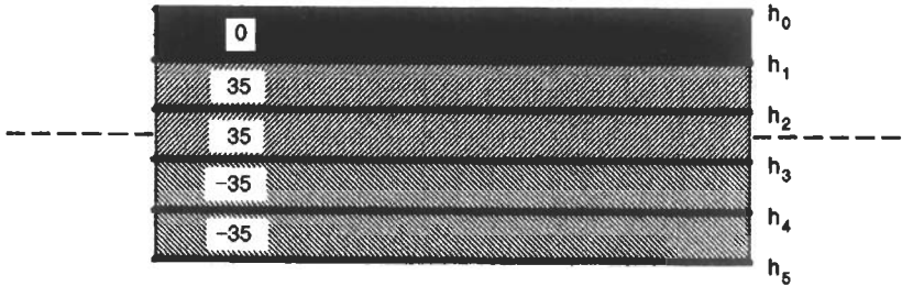
Fig. 3.27 Non-symmetric laminate
