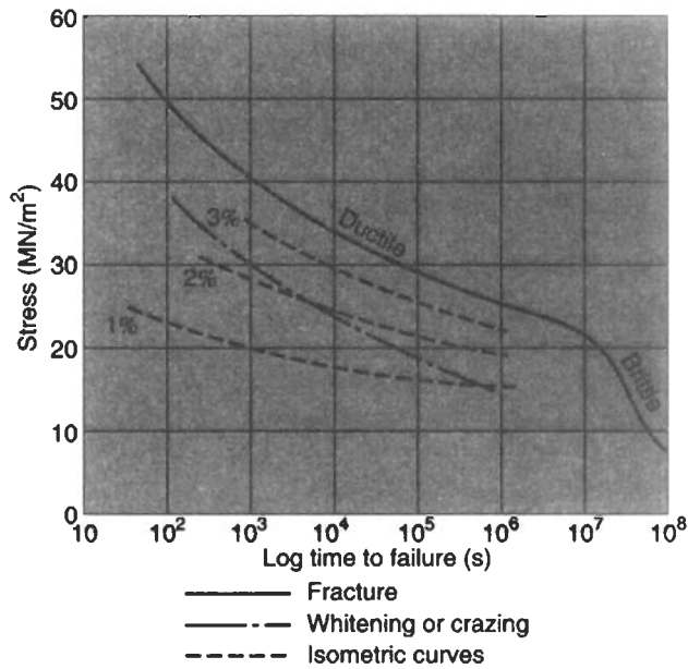
Fig. 2.71 Typical creep rupture behaviour of plastics
