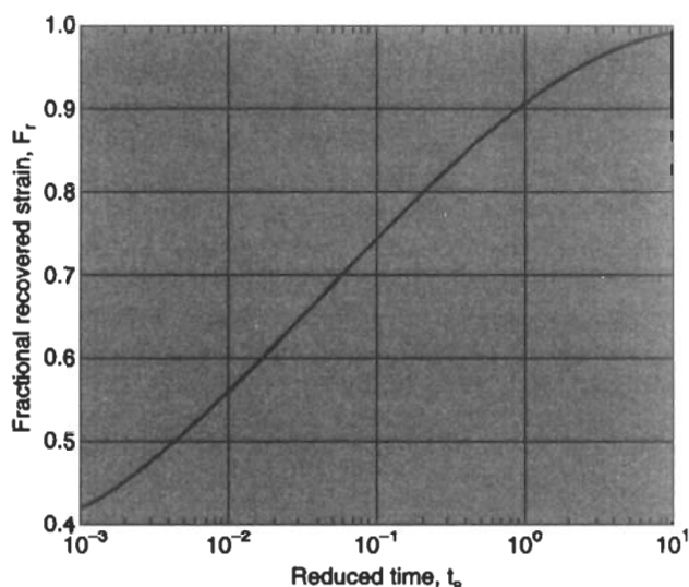
Fig. 2.50 Typical recovery behaviour of a plastic
