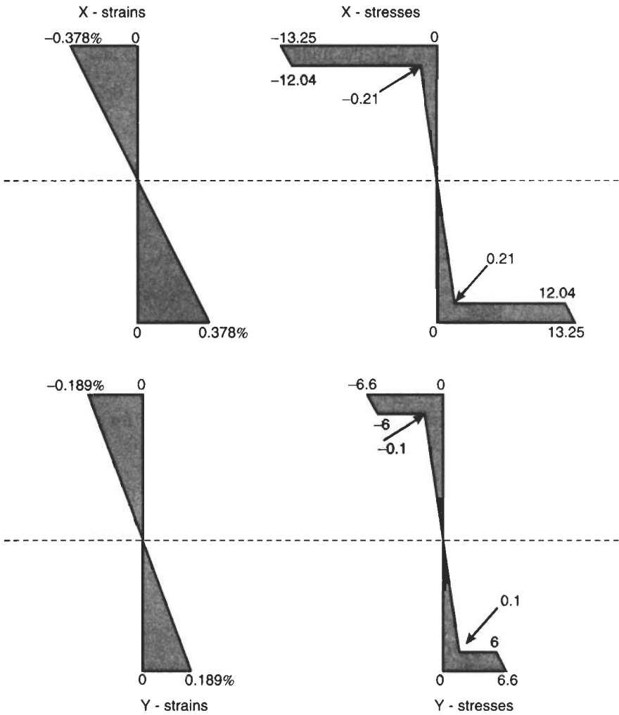
Fig. 3.26 Stresses and strains, Example 3.15
