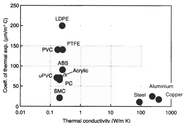
Fig. 1.11 Typical thermal properties of plastics
