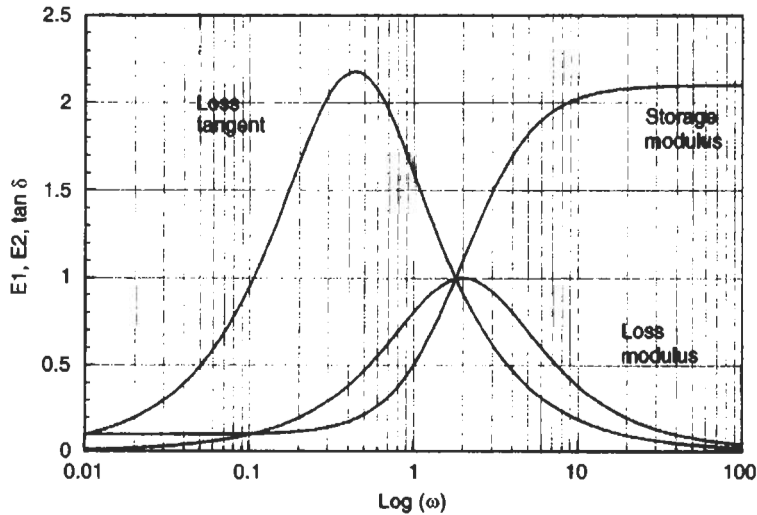
Fig. 2.57 Variation of E_1 , E_2 and loss tangent for standard linear solid
