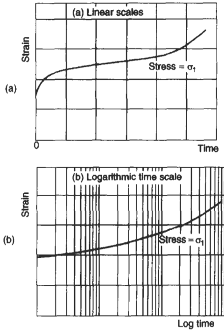
Fig. 2.4 Typical creep curves
