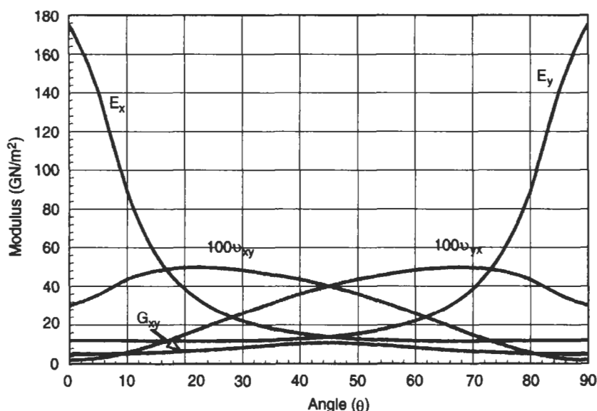
Fig. 3.24 Variation of elastic properties for a single ply of carbon/epoxy composite
