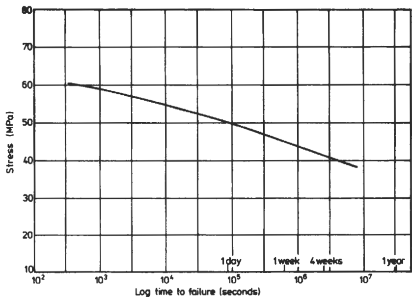
Fig. 2.90 Creep fracture of acetal
