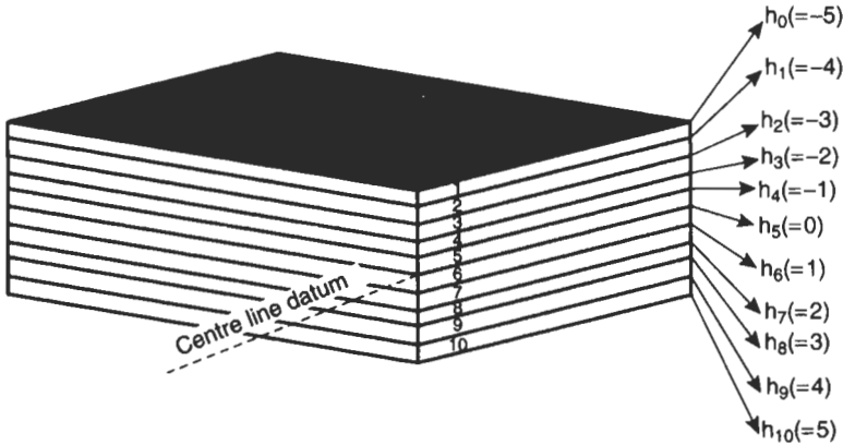
Fig. 3.22 Ten ply laminate
