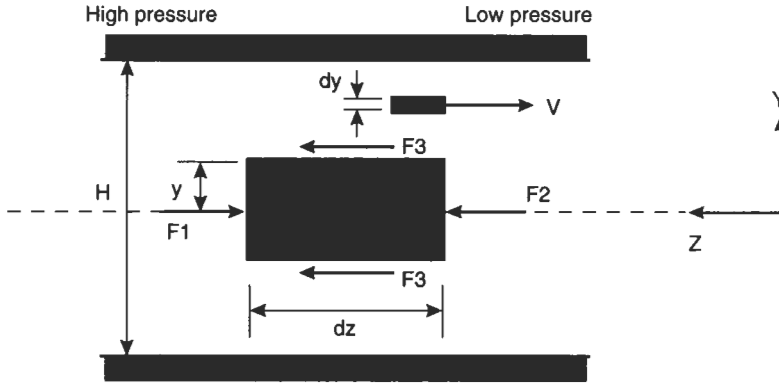
Fig. 5.5 Element of Fluid Between Parallel Plates
