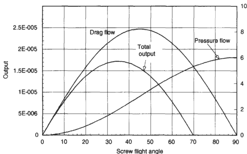
Fig. 4.10 Variation of drag flow and pressure flow
