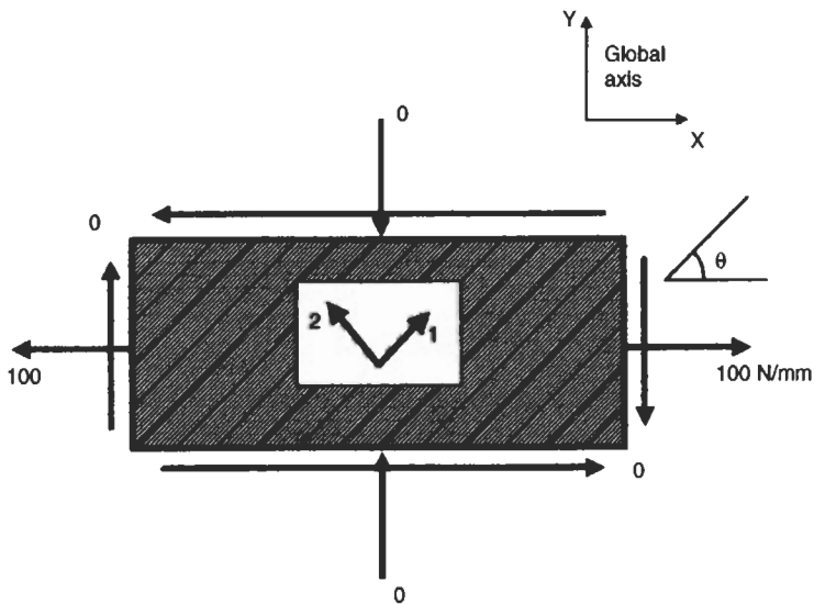
Fig. 3.16 Single ply composite subjected to plane stress
