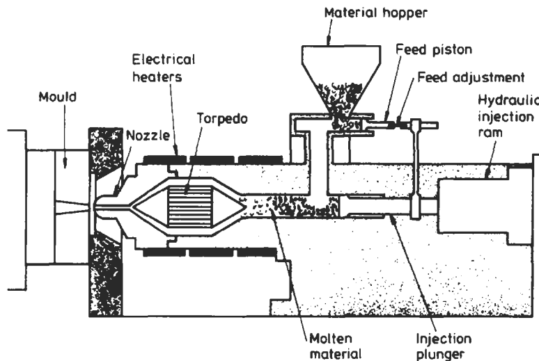
Fig. 4.30 Plunger type injection moulding machine
