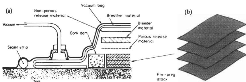
Fig. 4.69 Diagrammatic cross section of a bagged lay-up
