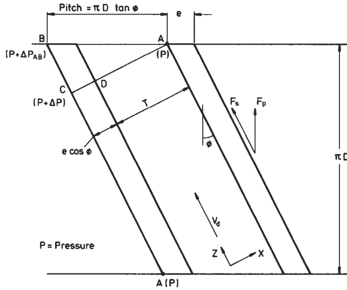
Fig. 4.9 Development of screw
