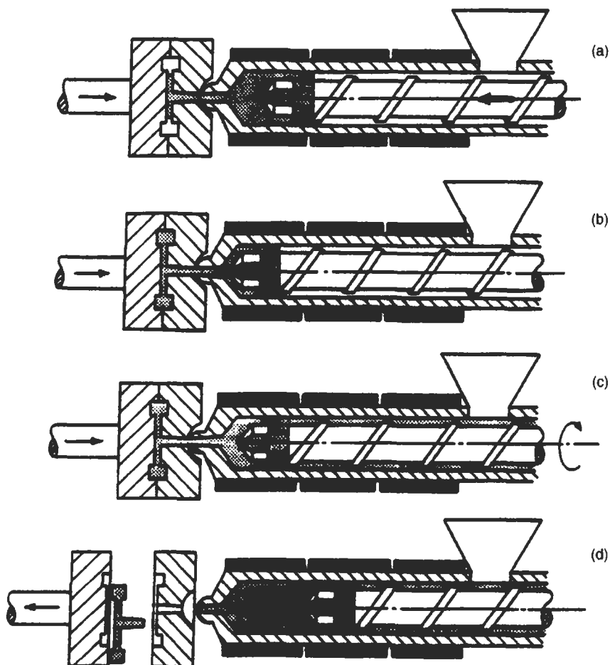
Fig. 4.31 Typical cycle in reciprocating screw injection moulding machine
