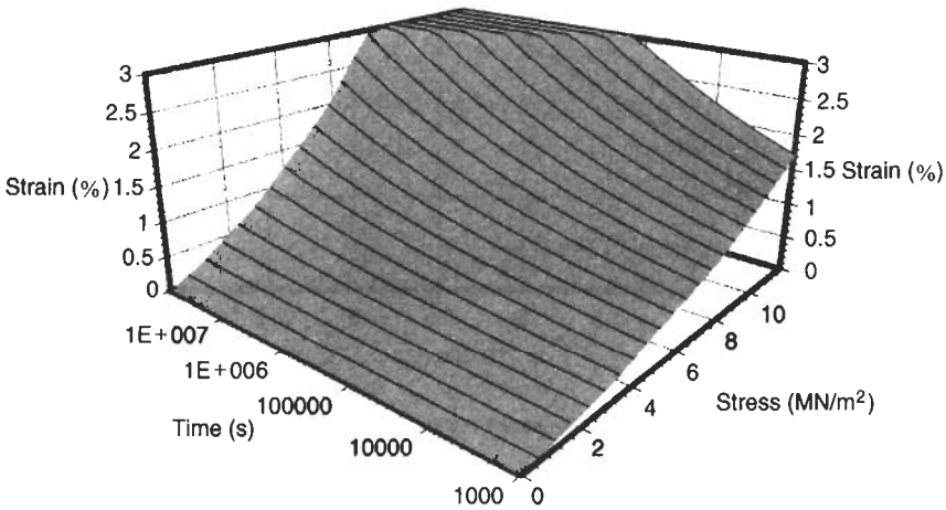
Fig. 2.6 Stress-strain-time curves for polypropylene
