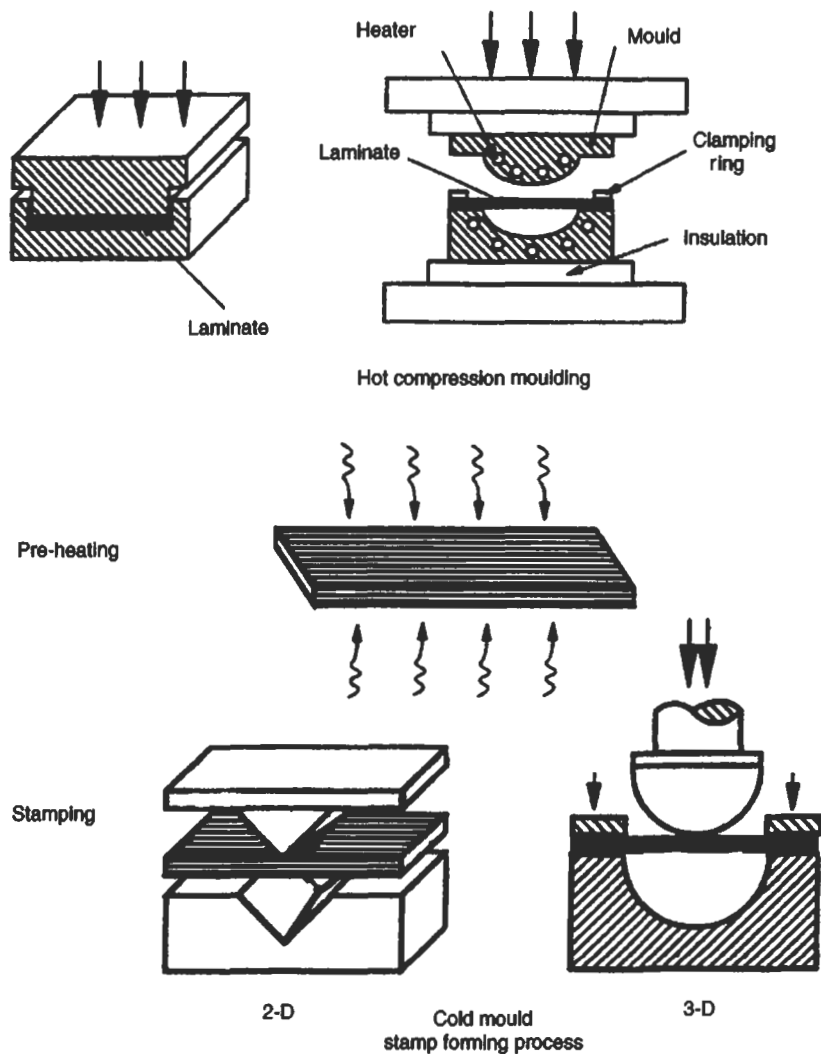
Fig. 4.73 Other types of compression moulding and stamp forming
