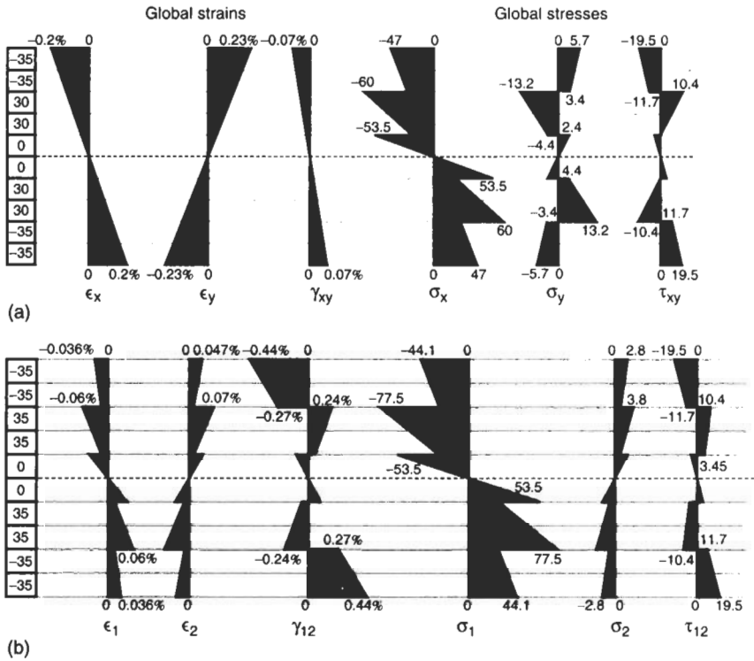
Fig. 3.23 Stresses and strains, Example 3.12: (a) global; (b) local
