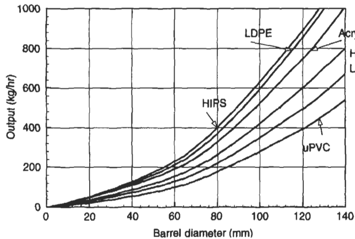
Fig. 4.3 Typical extruder outputs for different plastics
