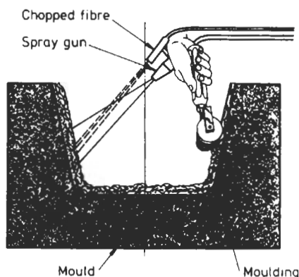
Fig. 4.68 Spray-up technique
