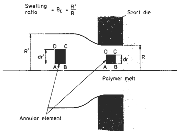
Fig. 5.12 Polymer Melt Emerging from a Short Die
