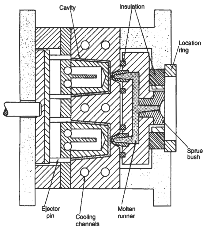
Fig. 4.39 Layout of hot runner mould
