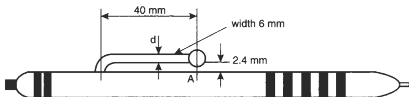
Fig. 2.11 Ball-point pen clip design
