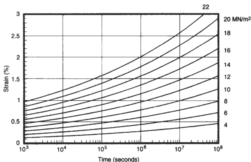
Fig. 2.15 Creep curves for acetal (20°C)
