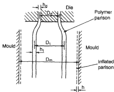
Fig. 4.23 Analysis of blow moulding
