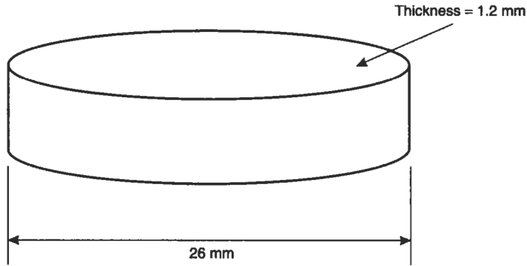
Fig. 2.14 Acetal bottle cap
