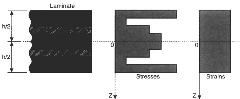
Fig. 3.19 Stresses and strains in a symmetric laminate
