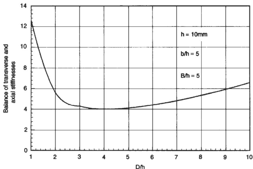
Fig. 2.32 Optimisation of corrugation depth
