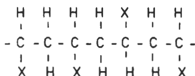
(a) Atactic
