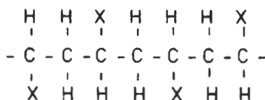
(b) Syndiotactic
