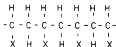
(c) Isotactic
