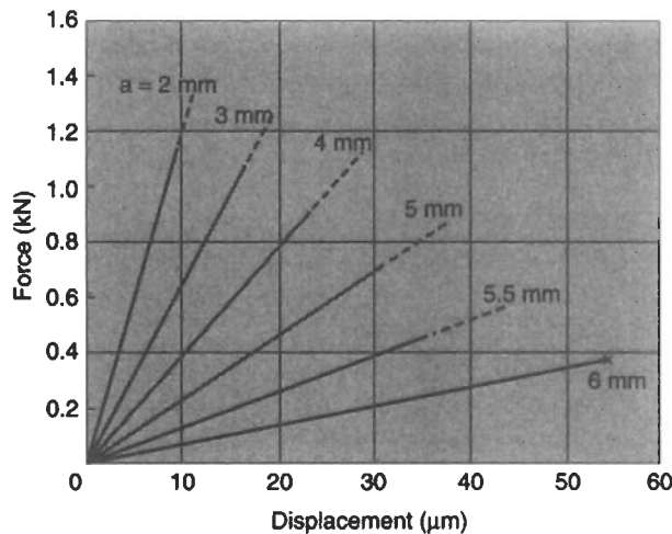
Fig. 2.64(a) Force-displacement characteristics for cracked plate
