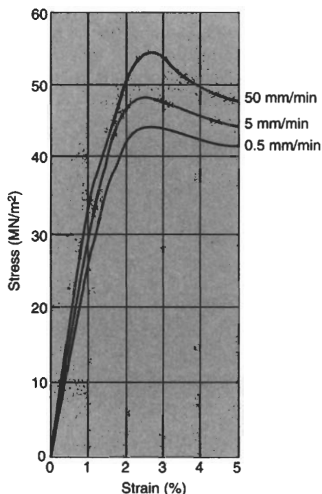
Fig. 1.4 Effect of strain rate on stress-strain behaviour of plastics
