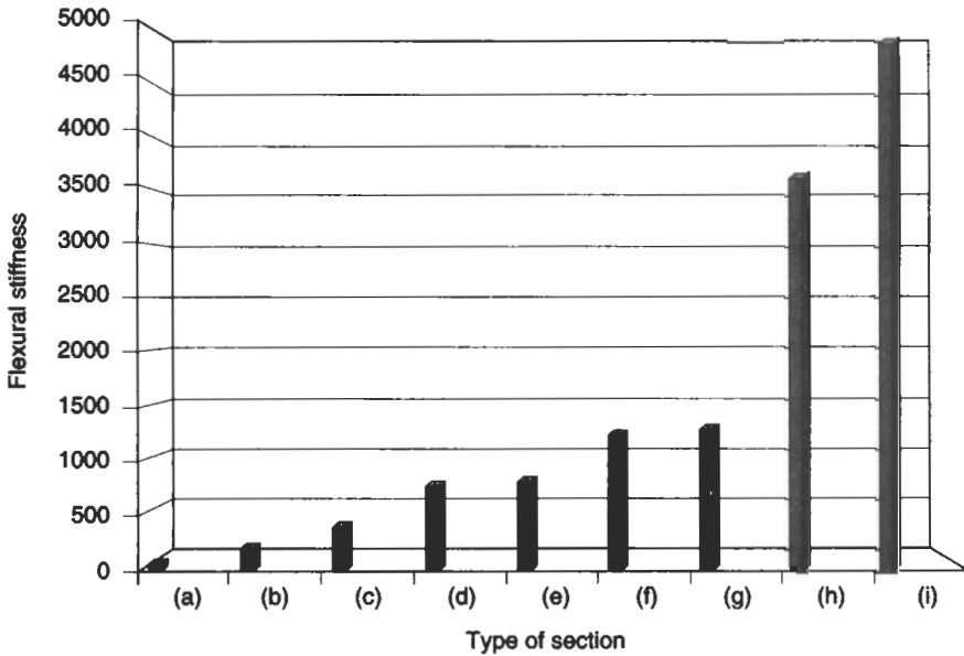
Fig. 2.26 Effect of geometry of flexural stiffness
