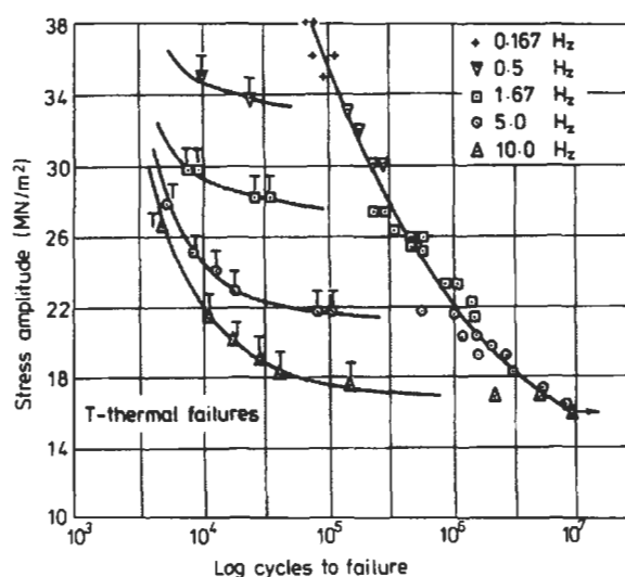
Fig. 2.75 Typical fatigue behaviour of acetal at several frequencies
