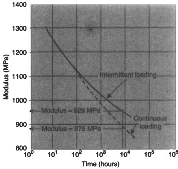
Fig. 2.52 Variation of modulus for continuous and intermittent loading
