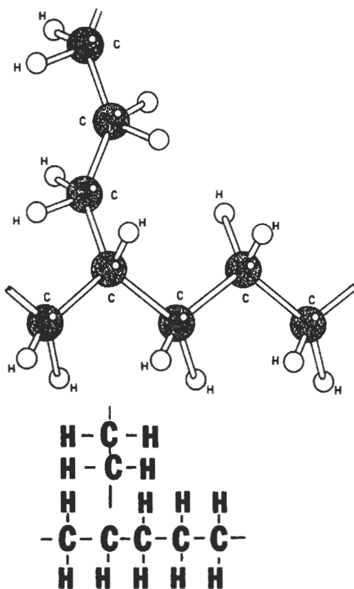
Fig. A.6 Chain branch in polyethylene
