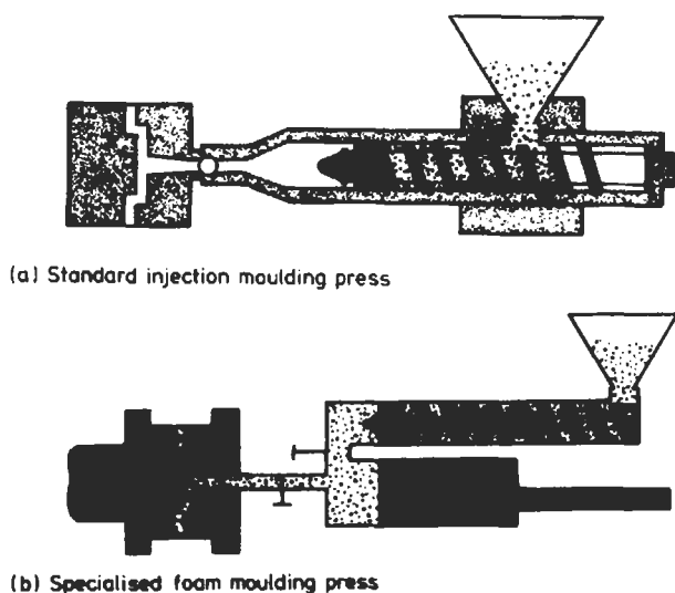
Fig. 4.43 Structural foam moulding equipment
