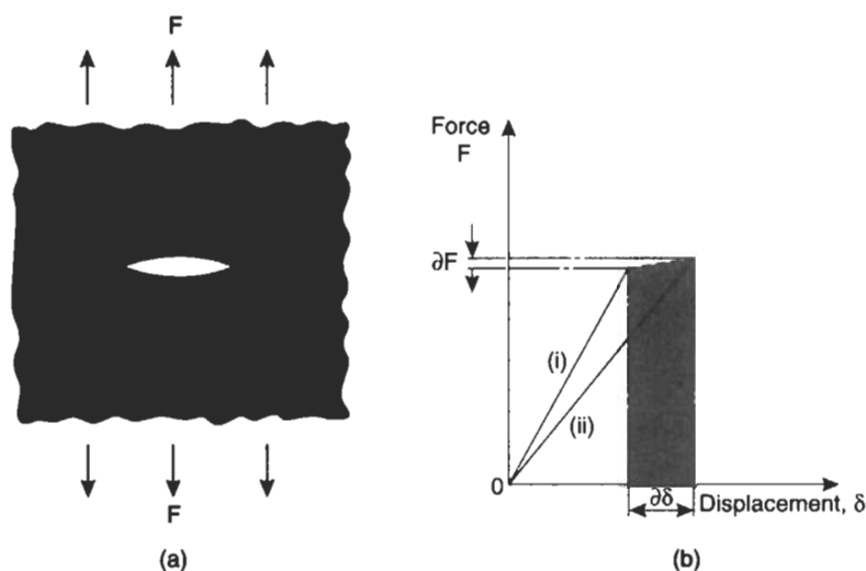
Fig. 2.63 Force displacement behaviour of an elastic cracked plate
