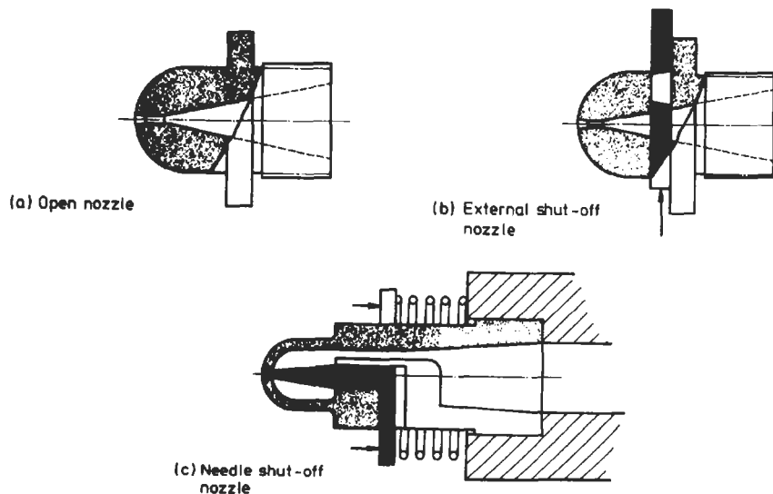
Fig. 4.34 Types of nozzle
