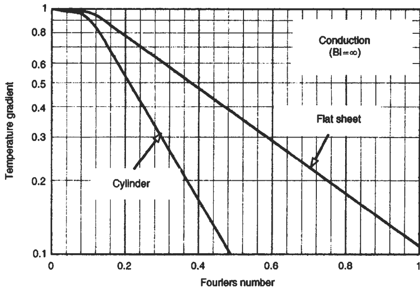
Fig. 5.23 Dimensionless Temperature Data for two Geometries
