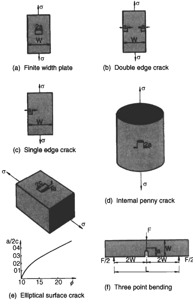
Fig. 2.67 Typical crack configurations
