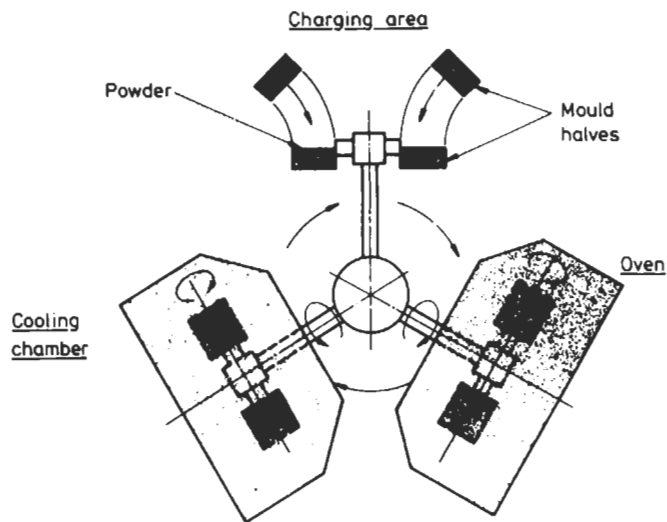
Fig. 4.59 Typical rotational moulding process
