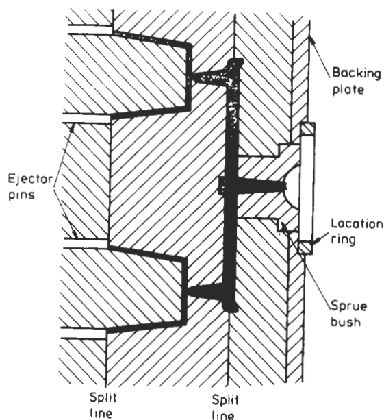
Fig. 4.38 Typical 3-plate mould
