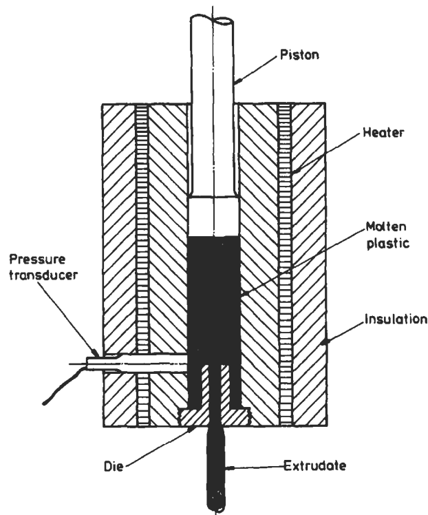
Fig. 5.16 Section Through Ram Extruder
