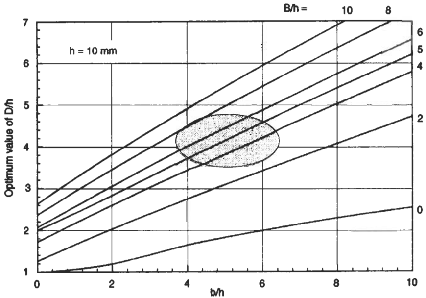
Fig. 2.33 Variation of optimum D/h with b/h
