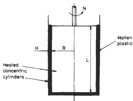
Fig. 5.15 Concentric Cylinder Viscometer
