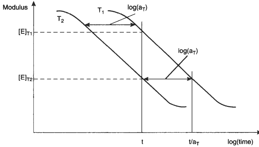
Fig. 2.59 Modulus curves at temperatures T_1 and T_2
