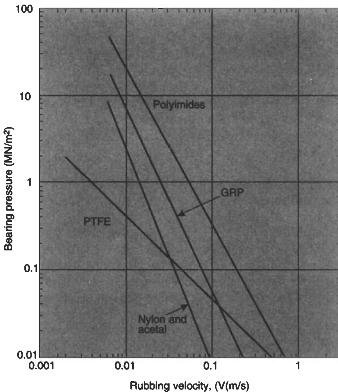
Fig. 1.9 Typical P-V ratings for plastics rubbing on steel
