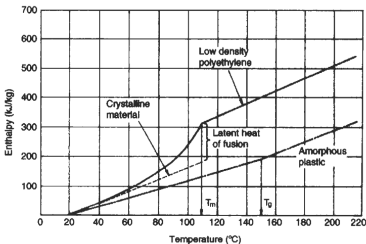
Fig. 5.29 Enthalpy Variation with Temperature
