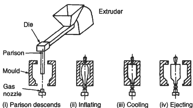
Fig. 4.21 Stages in blow moulding
