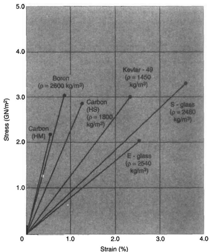
Fig. 3.2 Typical tensile behaviour of fibres
