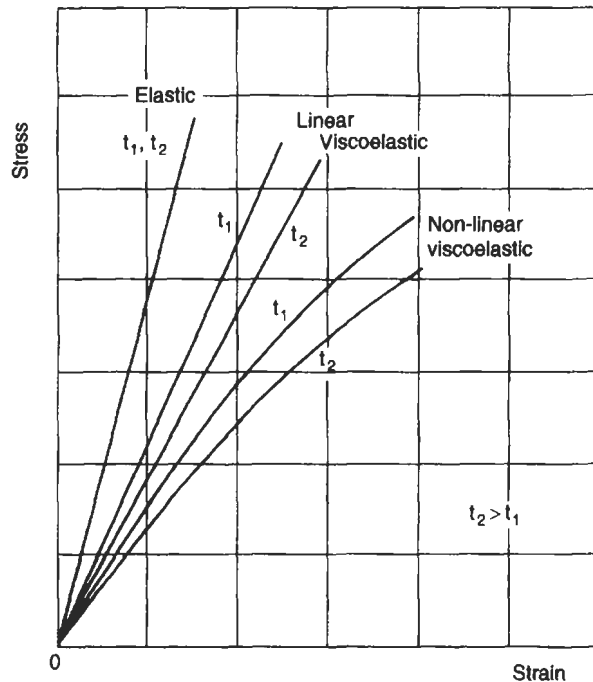
Fig. 2.1 Stress-strain behaviour of elastic and viscoelastic materials at two values of elapsed time, t
