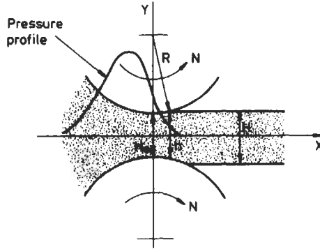
Fig. 4.58 Melt flow between calendar rolls
