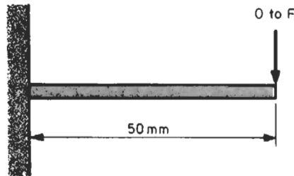
Fig. 2.88 Beam in timing mechanism
