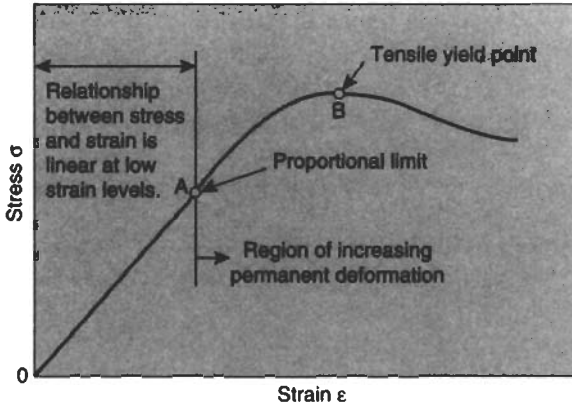
Fig. 1.2 Typical stress–strain graph for plastics
