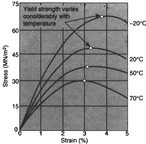
Fig. 1.3 Effect of material temperature on stress–strain behaviour of plastics
