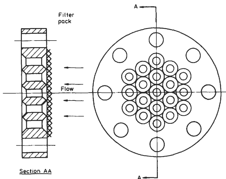
Fig. 4.6 Breaker plate with filter pack
