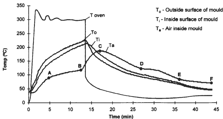
Fig. 4.61 Temperature profiles during rotational moulding
