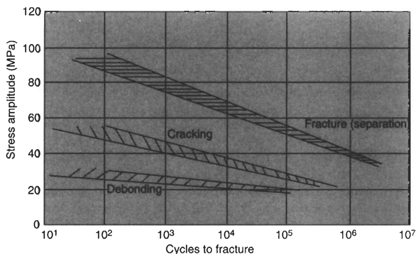
Fig. 3.32 Typical fatigue behaviour of glass reinforced polyester
