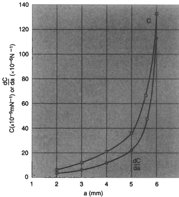
Fig. 2.64(b) Compliance and rate of change of compliance for various crack lengths
