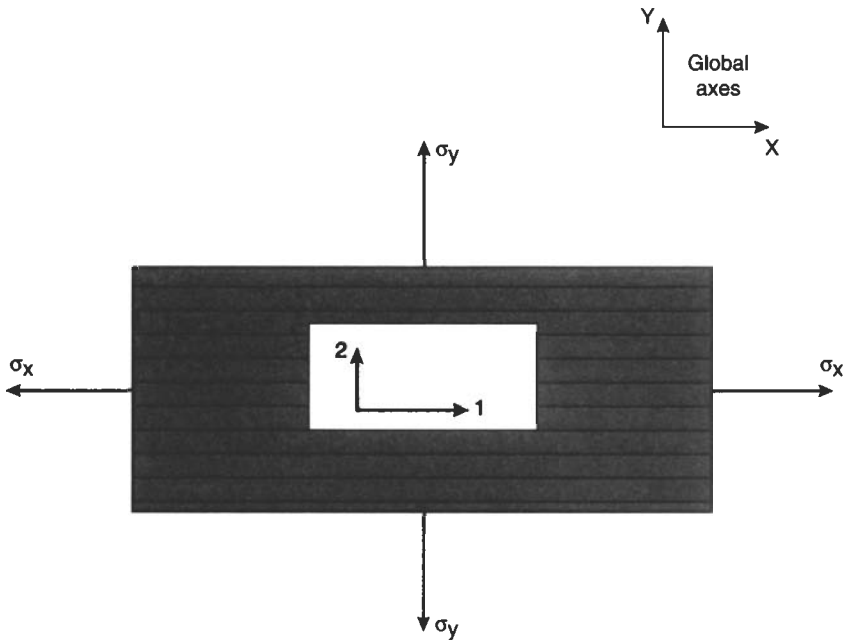
Fig. 3.9 Single thin lamina under plane stress
