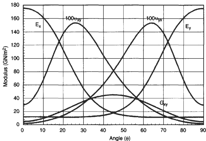
Fig. 3.25 Variation of elastic properties for a (+/- 45) symmetric laminate of carbon/epoxy
