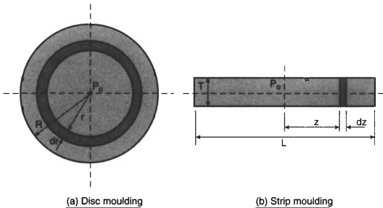
Fig. 4.41 Clamp force analysis
