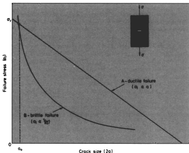
Fig. 2.68 Brittle and ductile failure characteristics for plastics
