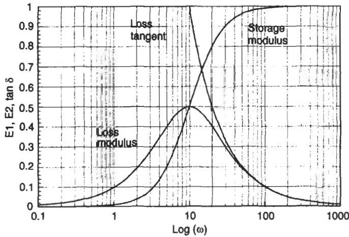
Fig. 2.56 Variation of E_1 , E_2 and loss tangent for Maxwell model
