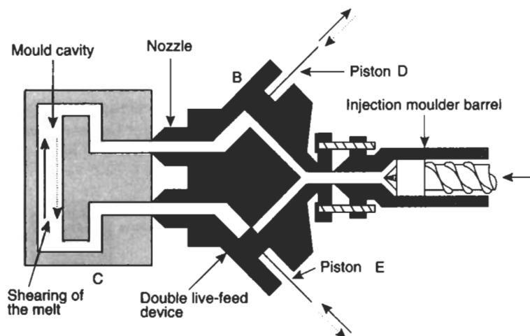
Fig. 4.46 One embodiment of SCORIM where the device (B) for producing shear during solidification, by the action of pistons (D) and (E), is placed between the injection moulding machine barrel (A) and the mould (C) (Courtesy of Brunel University)
