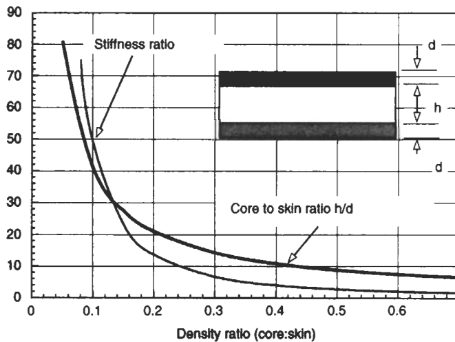
Fig. 2.21 Optimum skin to core ratio for constant weight
