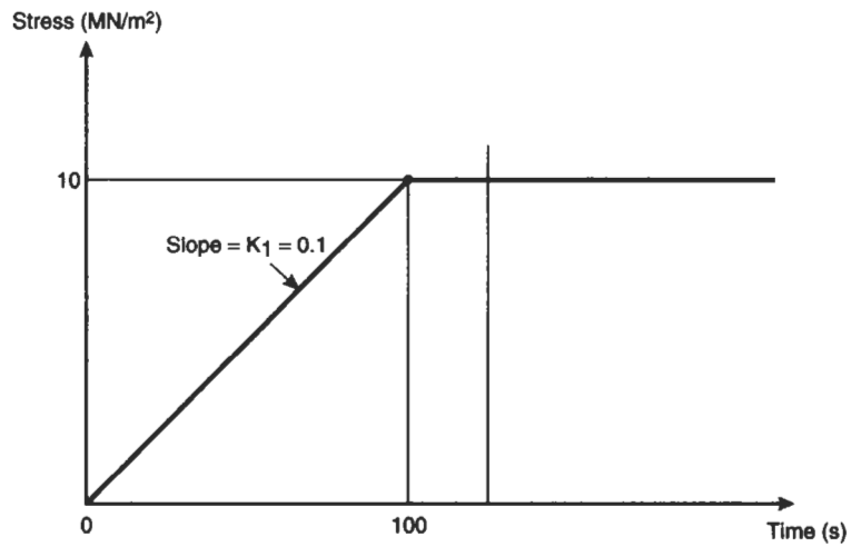
Fig. 2.47 Stress history: Example 2.15(a)
