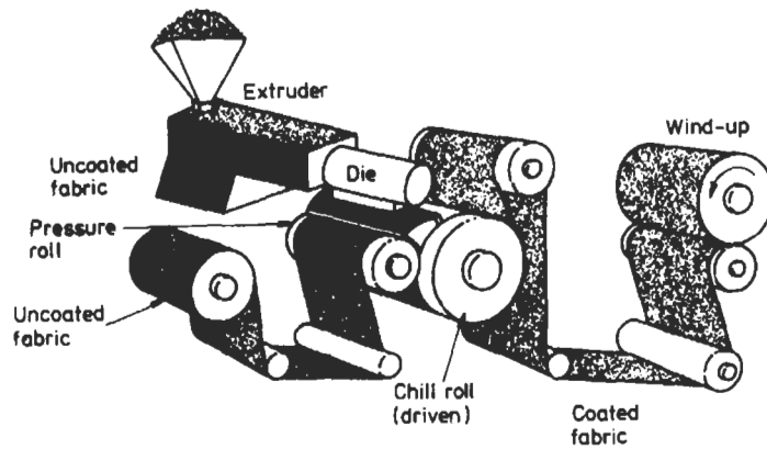
Fig. 4.26 Extrusion coating process
