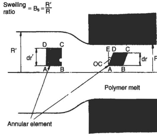
Fig. 5.10 Polymer Melt Emerging from a Long Die
