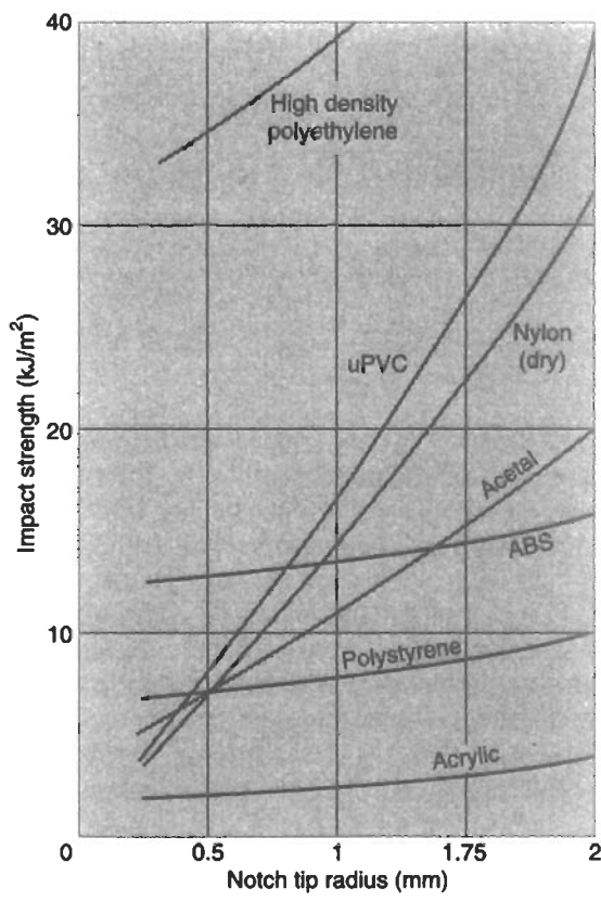
Fig. 2.79 Variation of impact strength with notch radius for several thermoplastics
