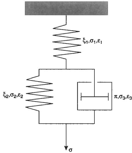
Fig. 2.86 Standard model for viscoelastic material
