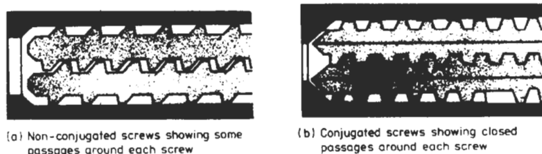
Fig. 4.15 Two types of twin screw extruder
