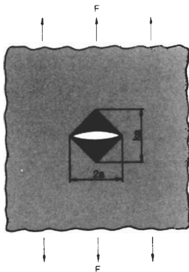
Fig. 2.65 Loading of cracked plate
