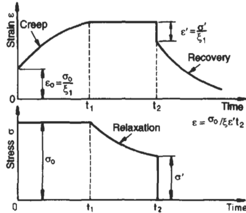
Fig. 2.39 Response of combined Maxwell and Kelvin models
