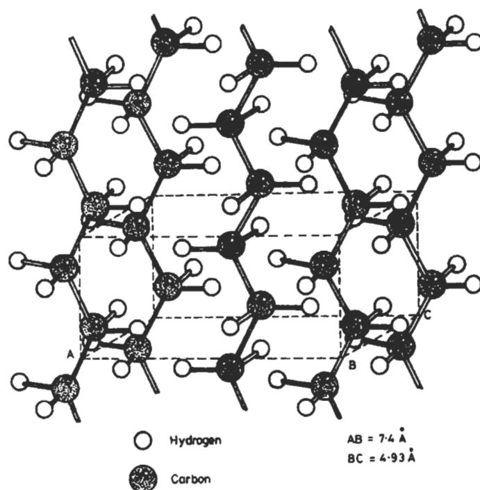
Fig. A.9 Crystalline structure of polyethylene
