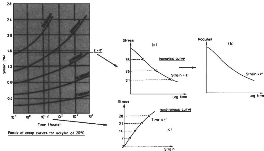
Fig. 2.10 Construction of isometric and isochronous graphs
