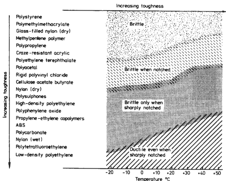
Fig. 2.82 Comparison of impact strengths as measured by Charpy test
