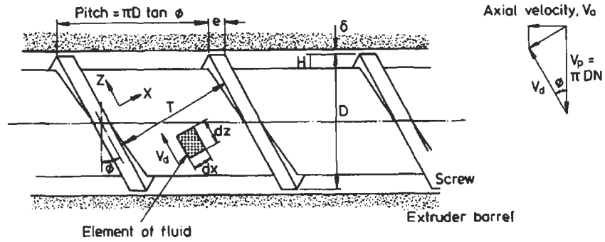
Fig. 4.8 Details of extruder screw
