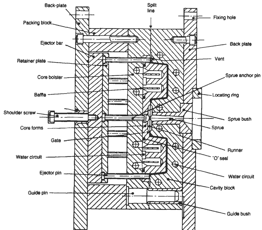
Fig. 4.35 Details of injection mould
