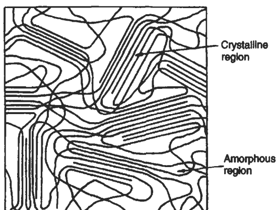
Fig. A.10 Fringed micelle model
