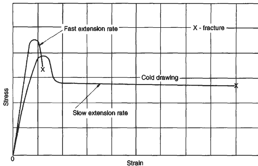
Fig. 2.2 Typical tensile behaviour of unplasticised PVC
