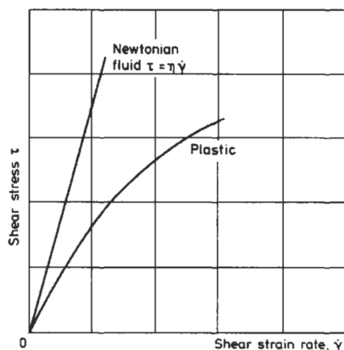
Fig. 5.1 Relations Between Shear Stress and Shear Rate
