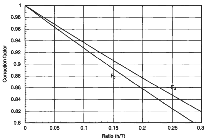
Fig. 4.11 Flow correction factors as a function of screw geometry
