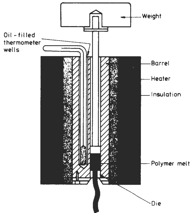
Fig. 5.18 Diagram of Apparatus for Measuring Melt Flow Index
