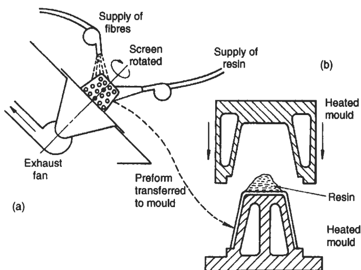
Fig. 4.71 Pre-form moulding of GFRP
