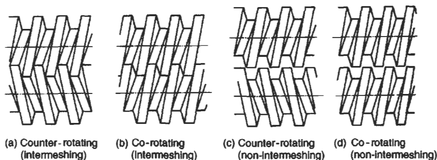
Fig. 4.14 Different types of twin screw extruder
