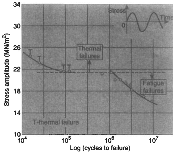
Fig. 2.74 Typical fatigue behaviour of acetal at 5 Hz
