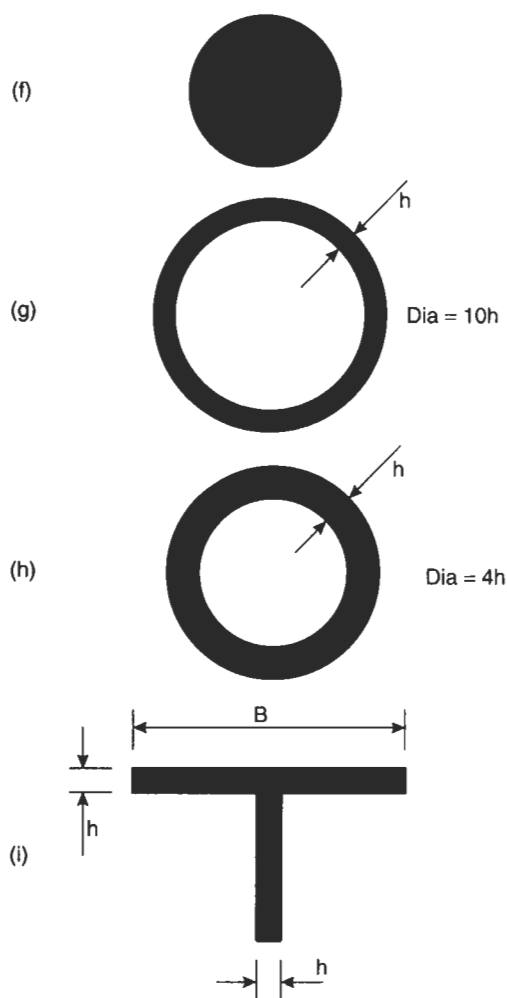
Fig. 2.25 (continued)
