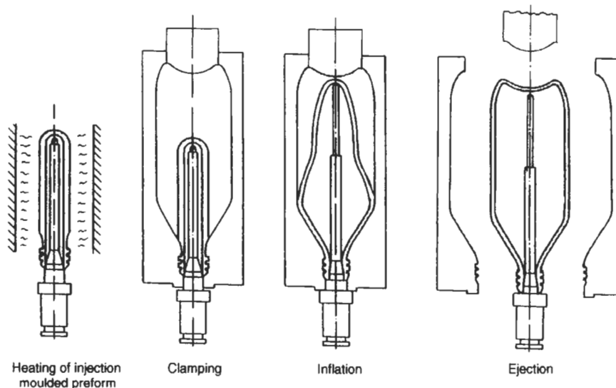
Fig. 4.48 Injection blow moulding process
