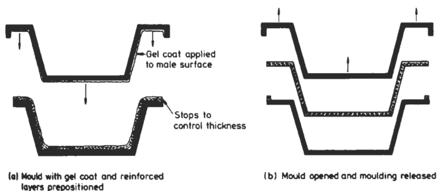
Fig. 4.70 Basic cold press moulding process
