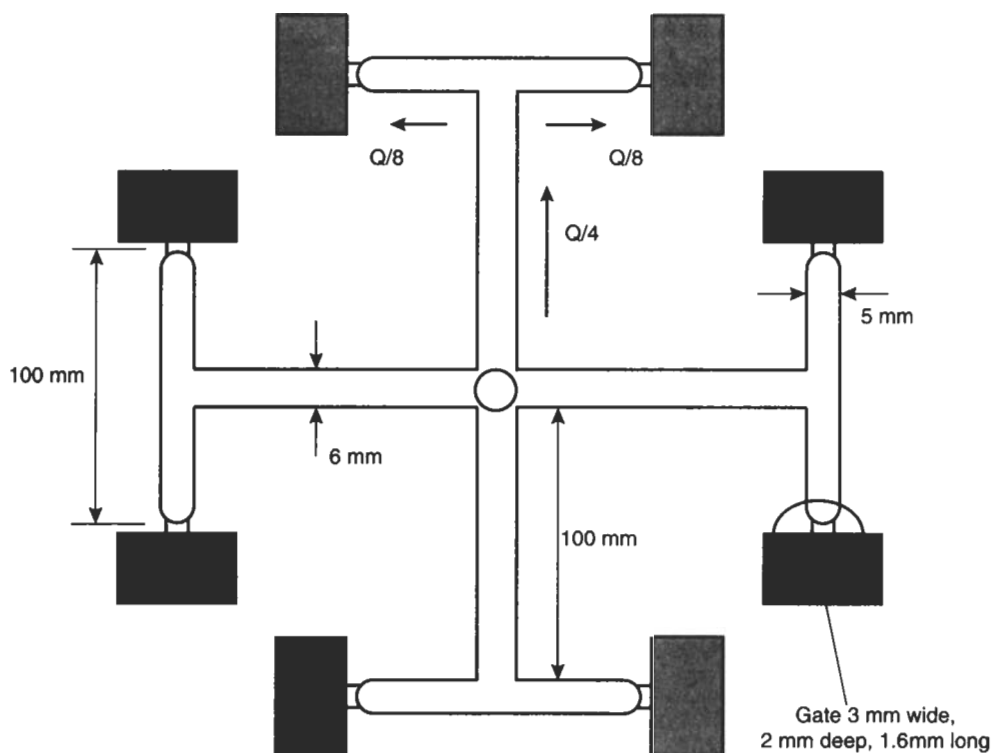
Fig. 5.19 Runner Layout, Example 5.4
