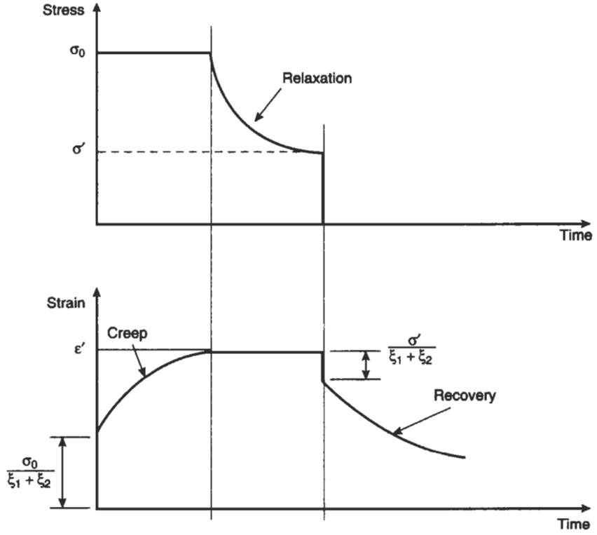
Fig. 2.42 Response of standard linear solid
