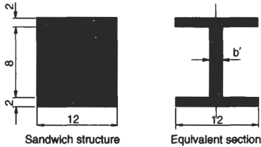
Fig. 2.18 Equivalent section for sandwich moulding
