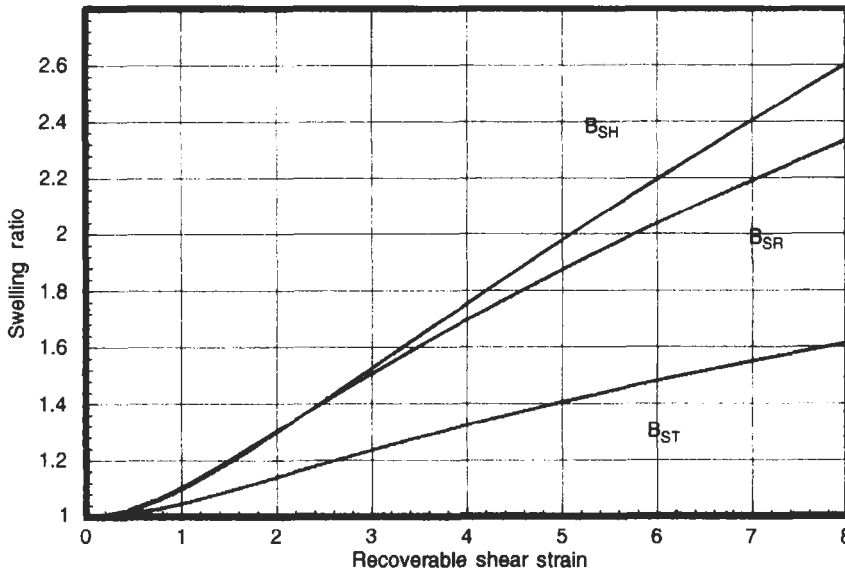
Fig. 5.11 Variation of Swelling Ratio for Capillary and Slit Dies
