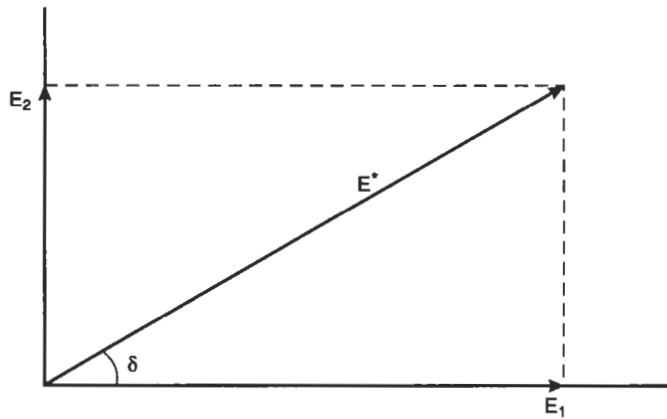
Fig. 2.54 Phasor diagram showing complex modulus ( E^* ) relative to loss ( E_2 ) and storage ( E_1 ) moduli
