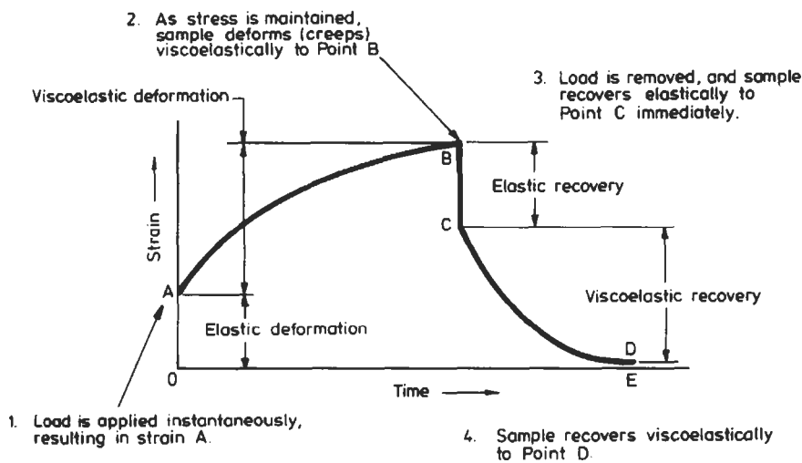
Fig. 1.8 Typical Creep and recovery behaviour of a plastic
