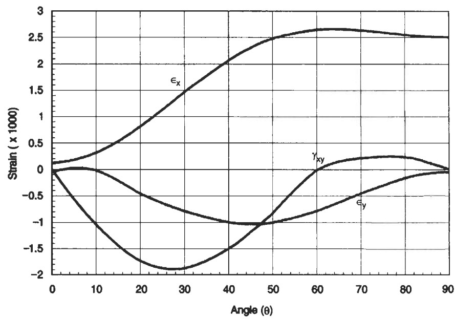
Fig. 3.13 Variation in direct and shear strains for unidirectional composite loaded axially
