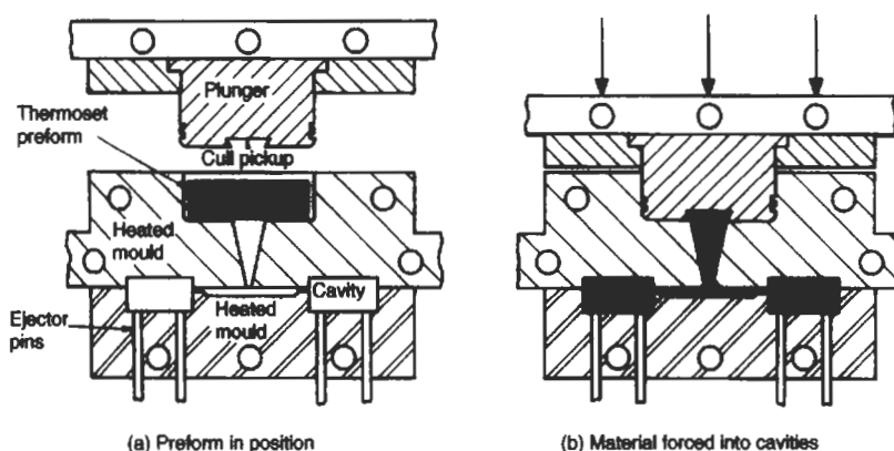
Fig. 4.64 Transfer moulding of thermosetting materials
