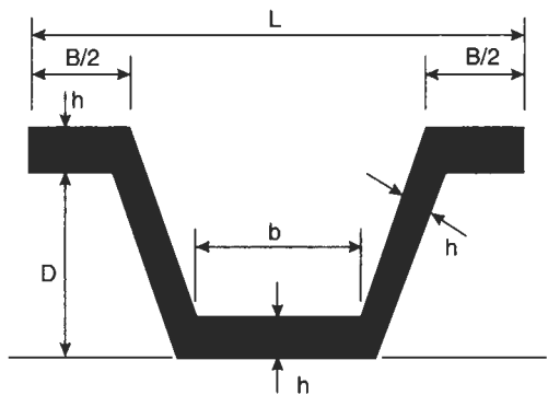
Fig. 2.30 Corrugation profile
