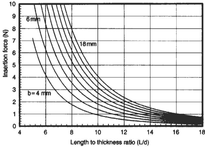
Fig. 2.23 Variation of insertion force with beam dimensions
