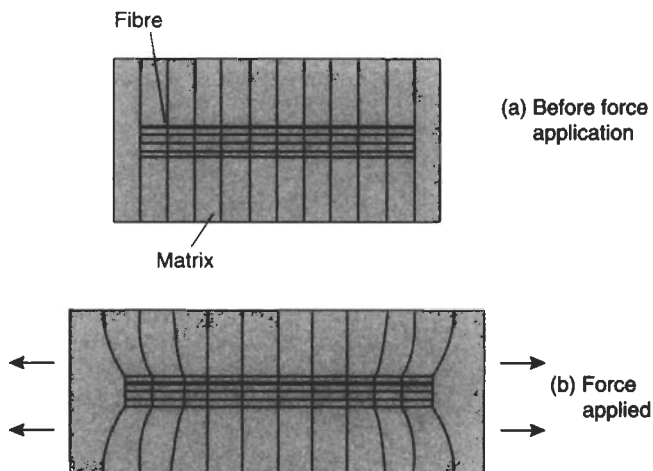
Fig. 3.28 Effect of fibre on deformation of matrix
