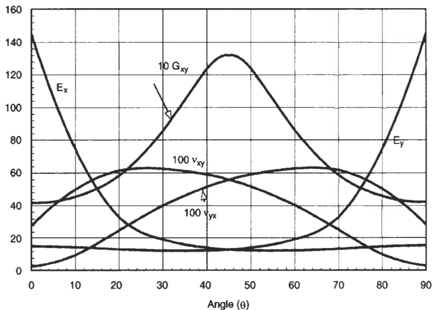
Fig. 3.11 Variation of properties in unidirectional composite as a function of fibre angle
