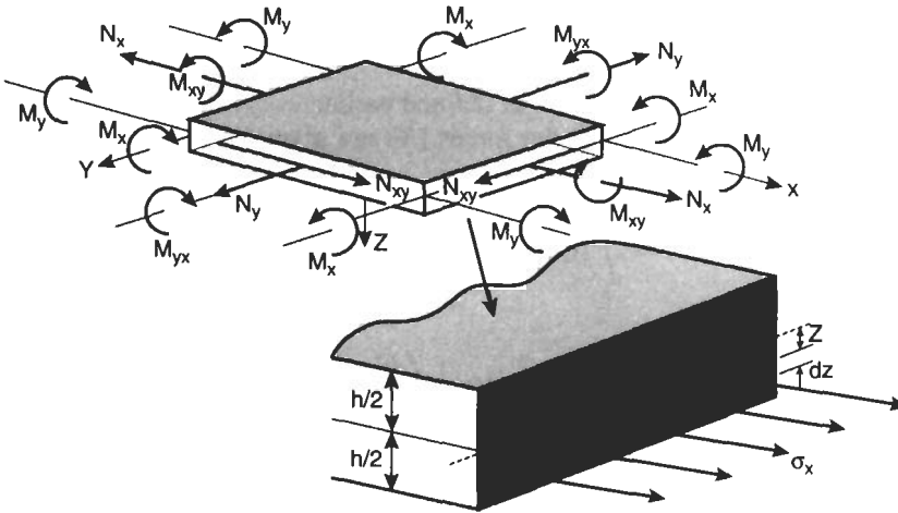
Fig. 3.15 General forces and moments acting on a single ply
