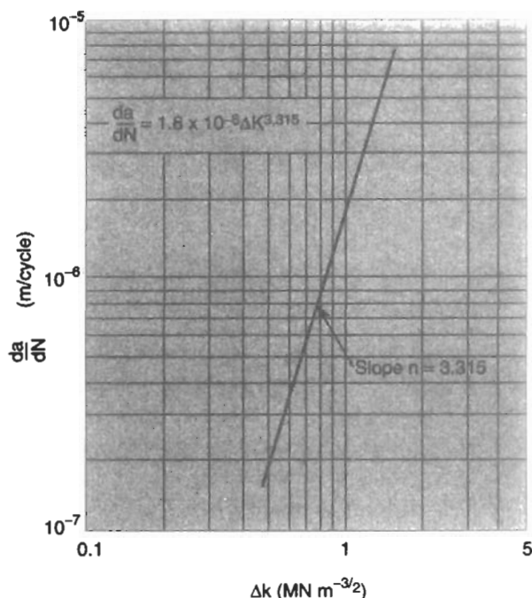
Fig. 2.77 Crack growth rate as a function of stress intensity factor
