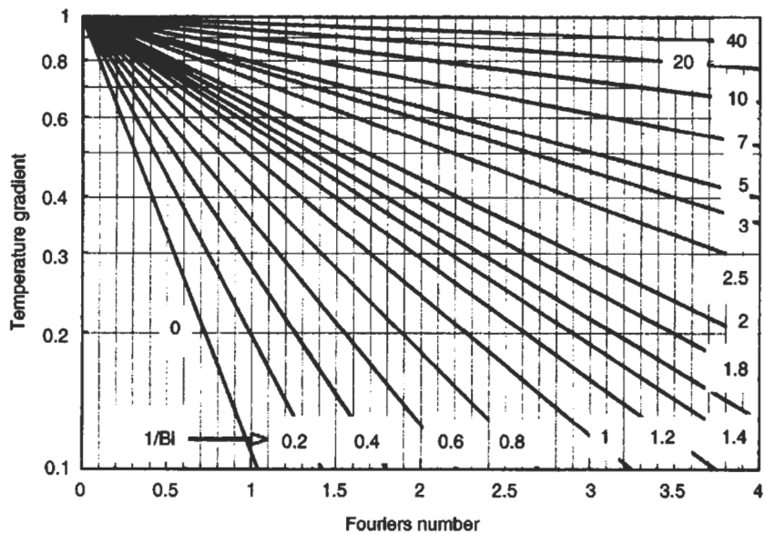
Fig. 5.24 Dimensionless Temperature Data for a Flat Sheet (Conduction/Convection)
