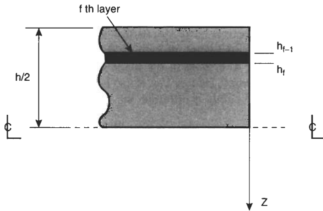
Fig. 3.20 Ply f in the laminate
