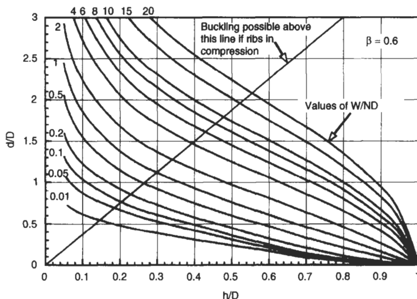
Fig. 2.28 Design of ribbed plates
