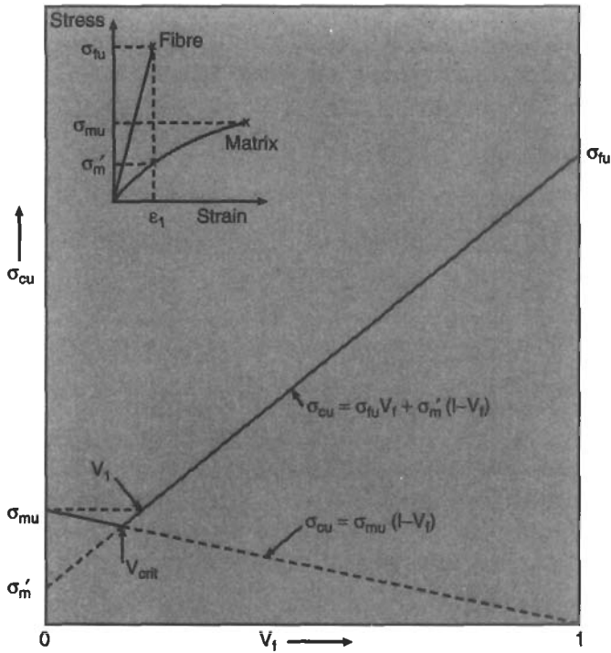
Fig. 3.5 Effect of volume fraction on strength
