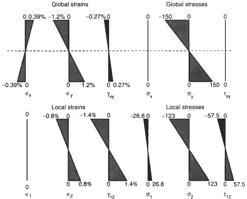
Fig. 3.18 Stresses and strains, Example 3.10
