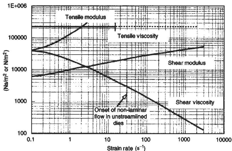
Fig. 5.3 Flow curves for polyethylene at 170°
