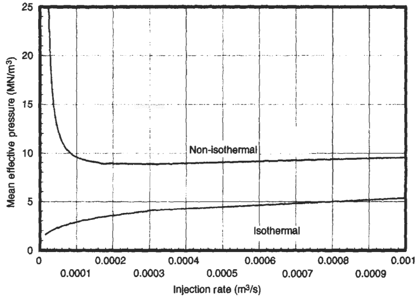
Fig. 5.28 Variation of Cavity Pressure Loss with Injection Rate
