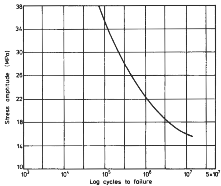
Fig. 2.89 Fatigue behaviour of acetal
