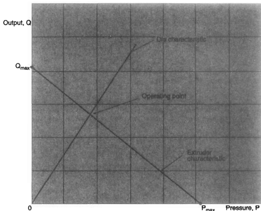
Fig. 4.12 Extruder and die characteristics
