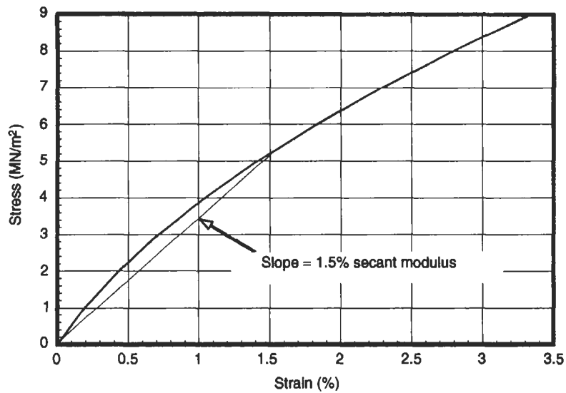
Fig. 2.13 Isochronous curve for polypropylene (1 year)
