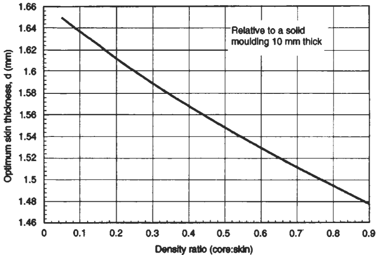
Fig. 2.20 Variation of optimum skin thickness with core: skin density ratio
