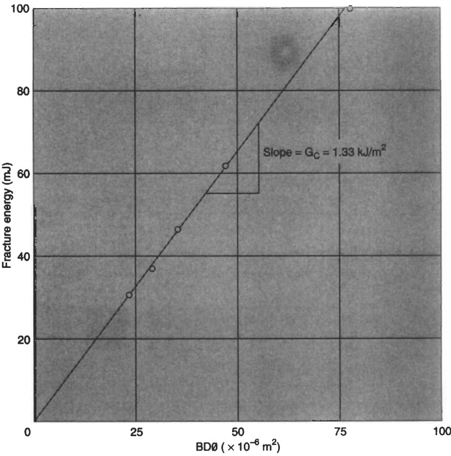
Fig. 2.84 Plot of U_c against BD\emptyset
