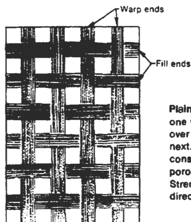
Fig. 4.65 Plain weave fibre fabric
