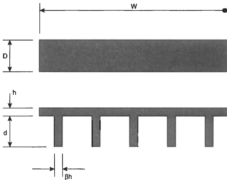
Fig. 2.27 Flat beam and ribbed section, Example 2.11
