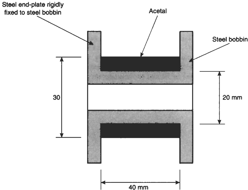
Fig. 2.16 Metal bobbin with plastic sleeve
