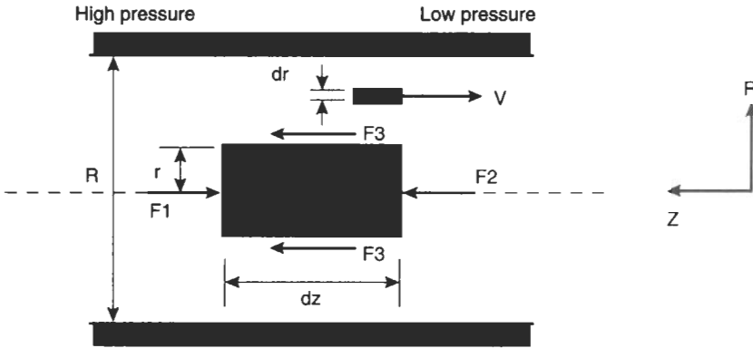
Fig. 5.4 Element of Fluid in a Capillary
