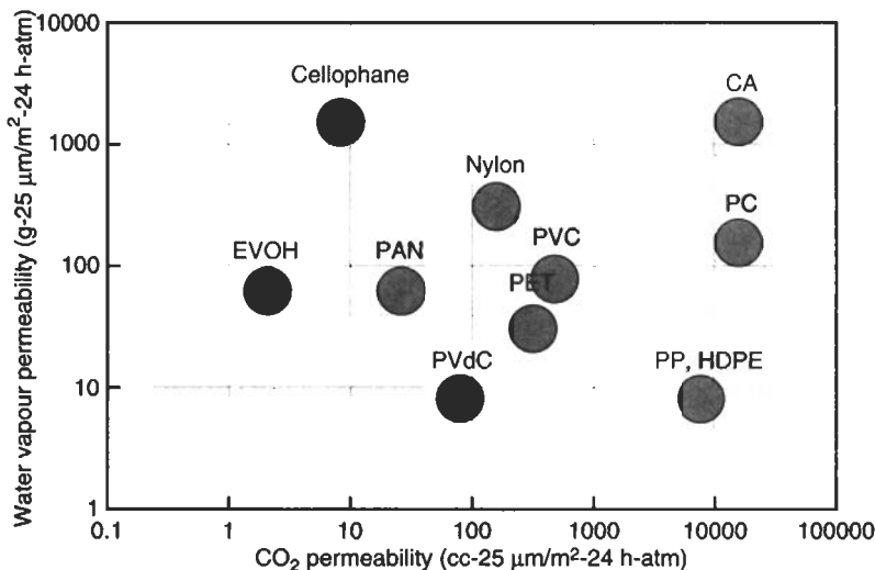
Fig. 1.14 Permeability data for a range of plastics
