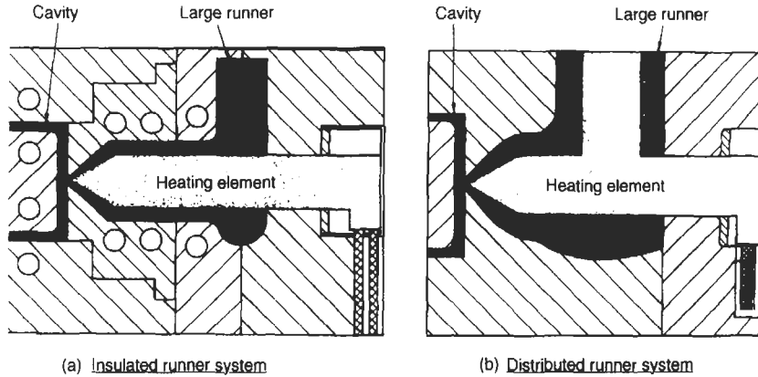
Fig. 4.40 Insulated and distributed runner systems
