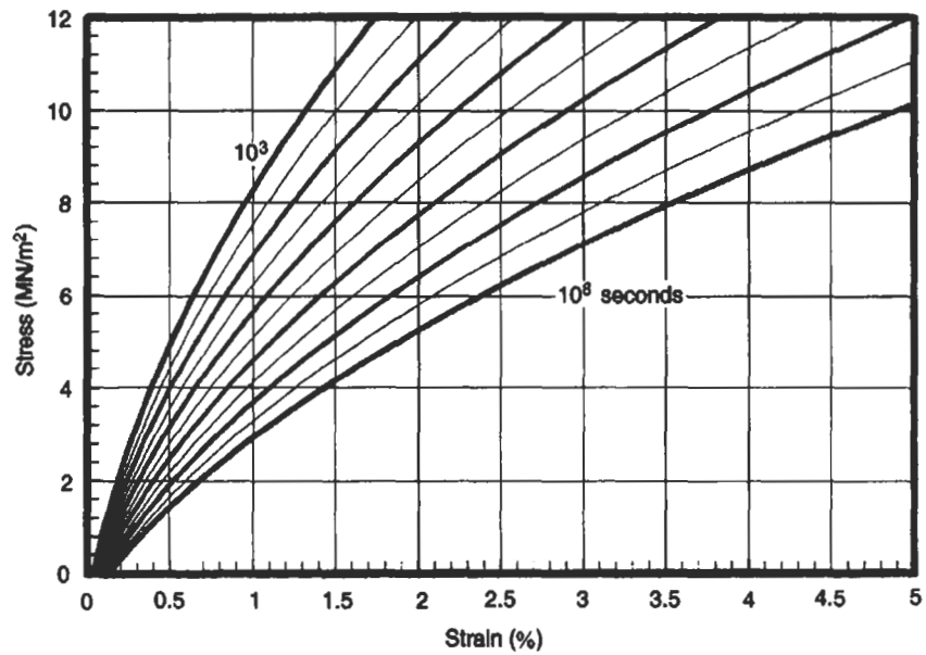
Fig. 2.7 Stress-strain curves for polypropylene
