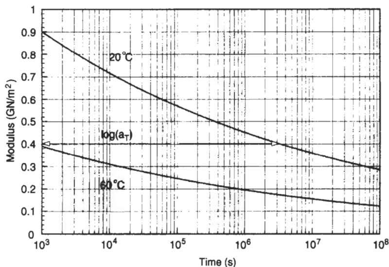
Fig. 2.61 Variation of modulus with time and temperature for polypropylene
