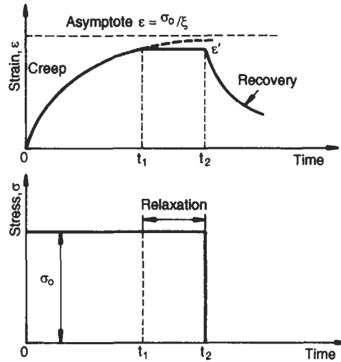
Fig. 2.37 Response of Kelvin/Voigt model
