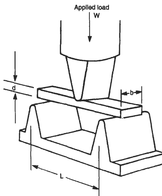
Fig. 2.3 Three-point bending
