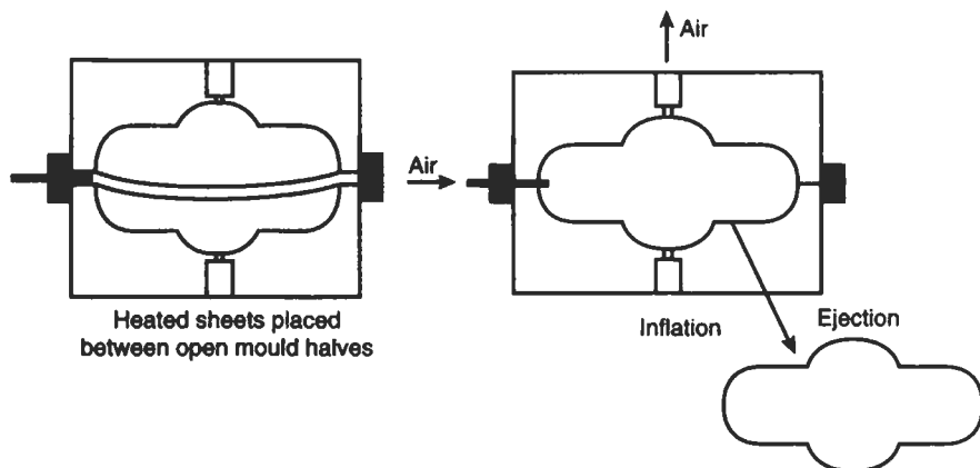
Fig. 4.54 Dual sheet forming
