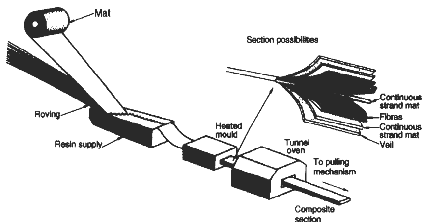
Fig. 4.77 Pultrusion process
