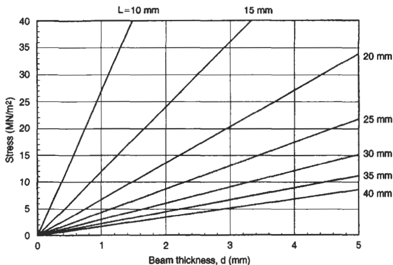
Fig. 2.24 Variation of stress with beam dimensions
