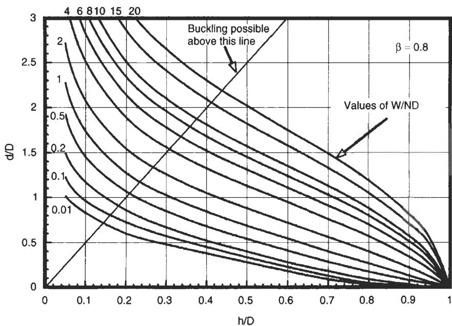
Fig. 2.29 Design of ribbed beams
