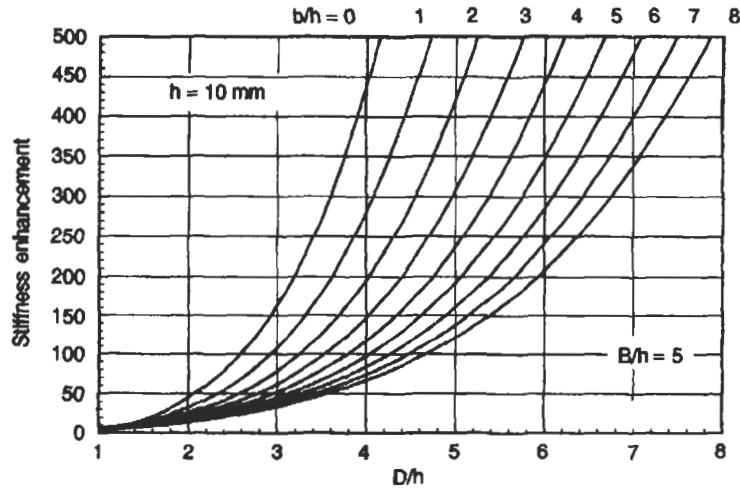
Fig. 2.31 Stiffness of corrugations as function of dimensions
