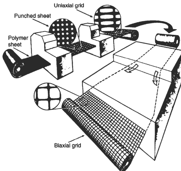
Fig. 4.29 Tensar manufacturing process
