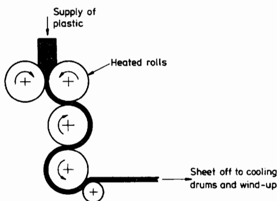
Fig. 4.57 Typical arrangement of calender rolls
