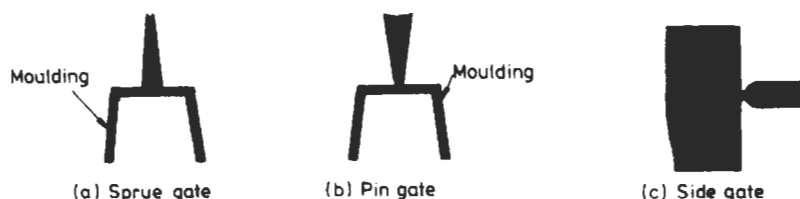
Fig. 4.36 Types of gate
