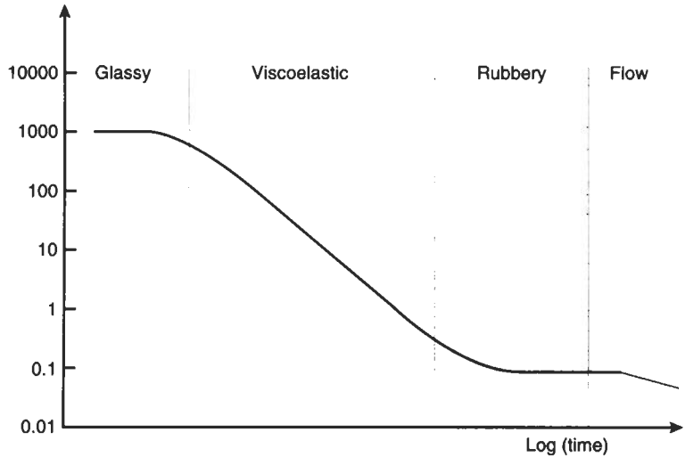
Fig. 2.9 Typical variation of creep or relaxation moduli with time
