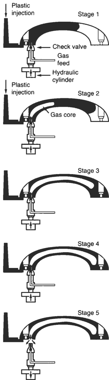
Fig. 4.45 Stages in the gas injection moulding of an automotive handle (courtesy of Cinpress Ltd)
