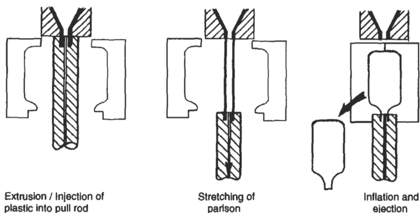
Fig. 4.24 Neck ring stretch blow moulding
