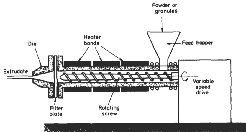
Fig. 4.1 Schematic view of single screw extruder
