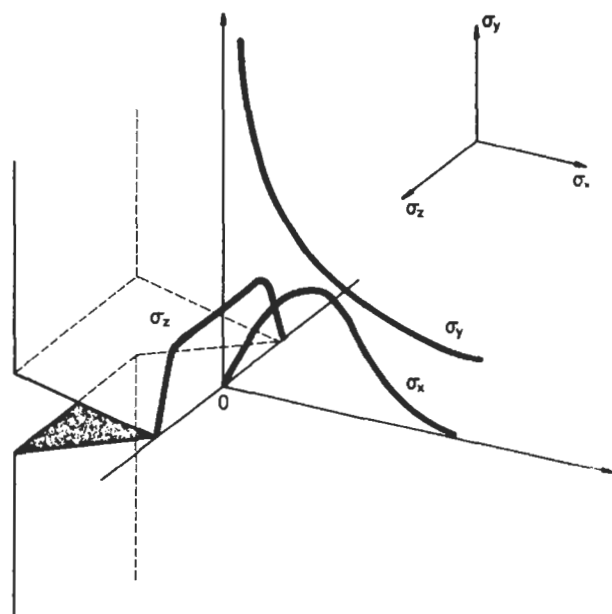
Fig. 2.78 Triaxial stress distribution at a notch
