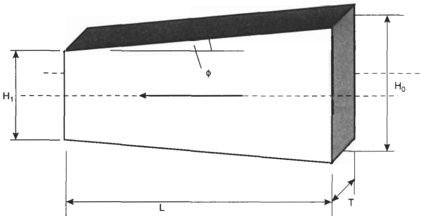
Fig. 5.9 Analysis of Flow in Tapered Wedge
