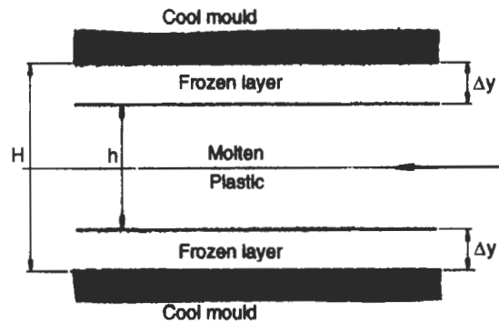
Fig. 5.25 Flow of Molten Polymer into a Cold Mould
