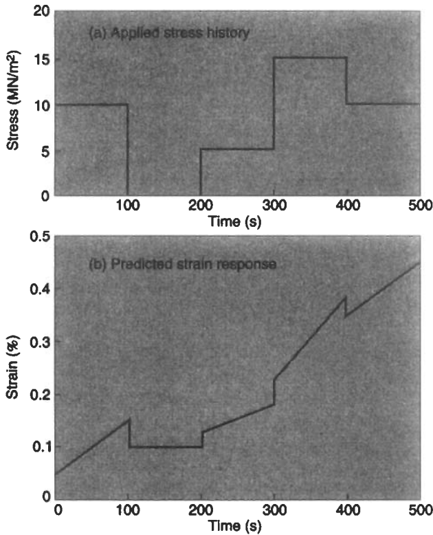
Fig. 2.43 Strain predictions using superposition theory
