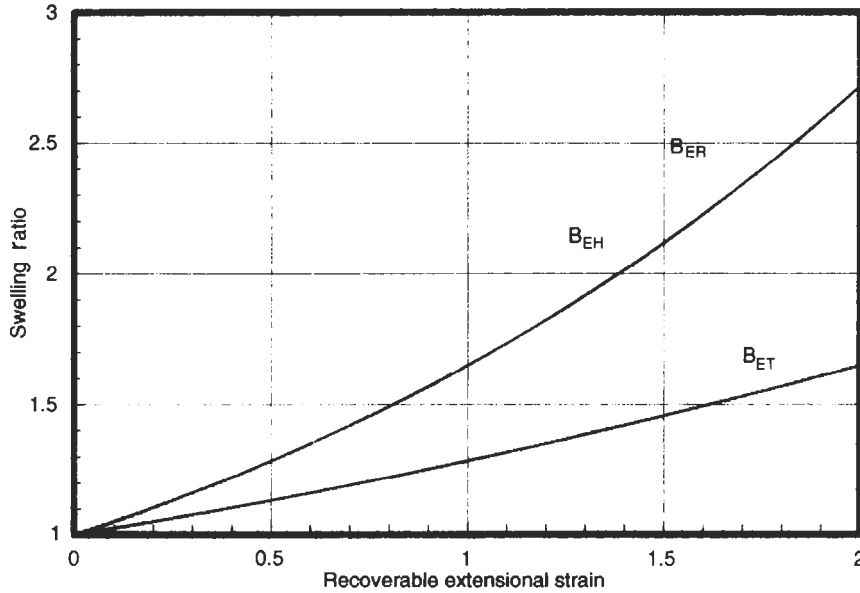
Fig. 5.13 Variation of Swelling Ratio for Capillary and Slit Dies
