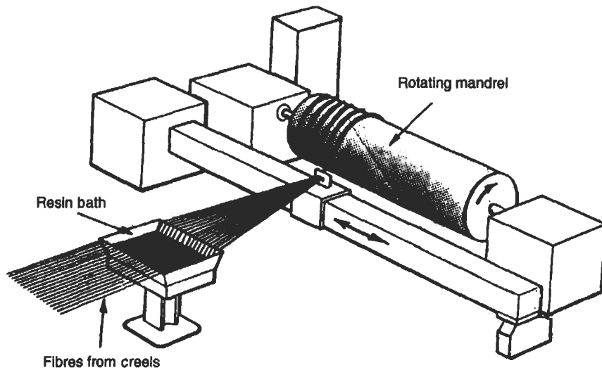
Fig. 4.75 Filament winding of fibre composites
