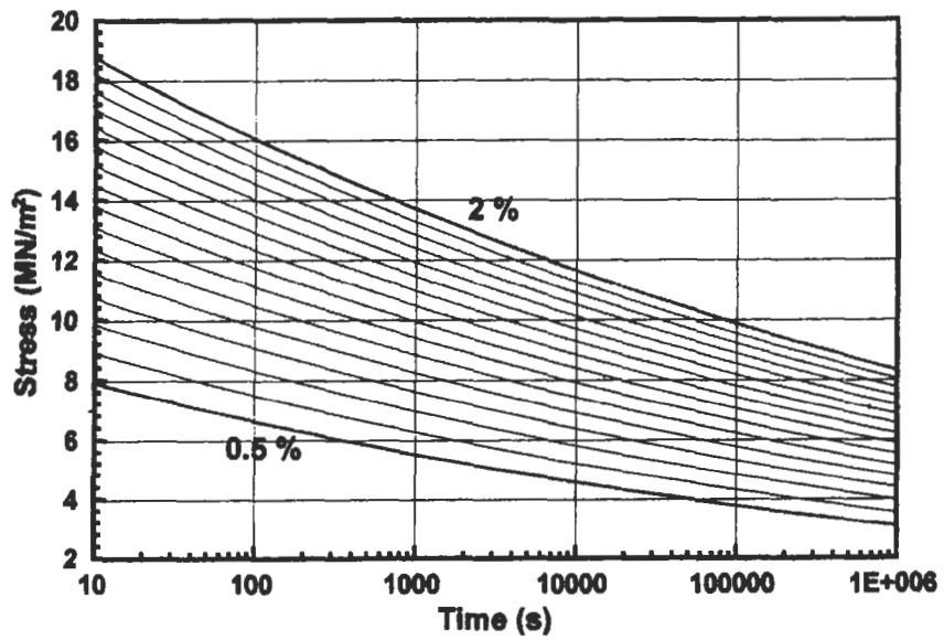
Fig. 2.8 Stress-time curves for polypropylene
