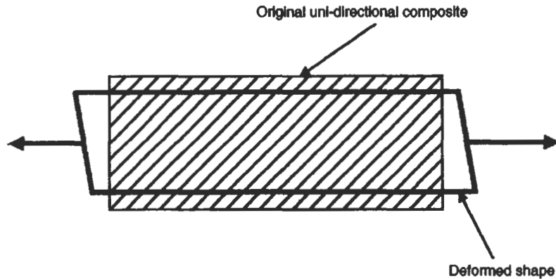
Fig. 3.17 Coupling effects between extension and shear
