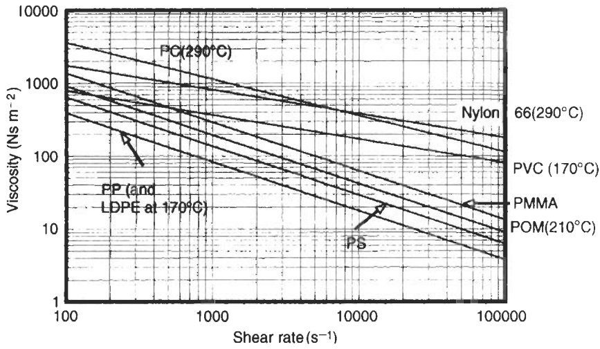
Fig. 5.17 Viscosity Curves for a Range of Plastics (230°C unless otherwise shown)
