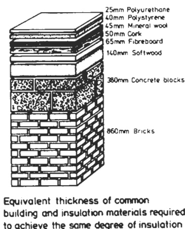
Fig. 1.10 Comparative Thermal conductivities for a range of materials
