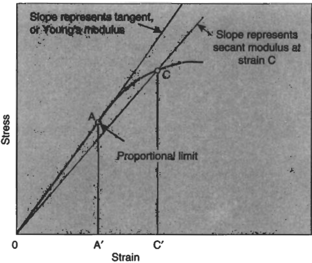
Fig. 1.6 Tangent and secant modulus
