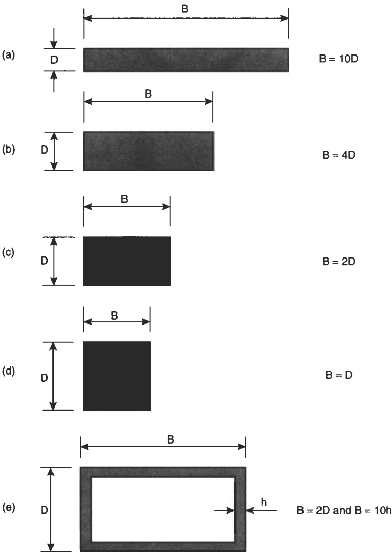
Fig. 2.25 Various cross-sections
