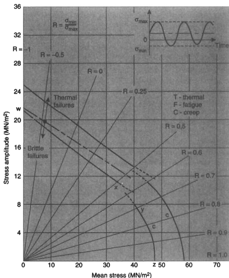
Fig. 2.76 Relationships between stress amplitude and mean stress
