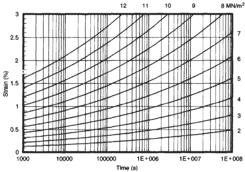
Fig. 2.5 Creep curves for polypropylene at 20°C (density 909 kg/m 3 )
