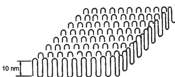
Fig. A.11 Folded chain model
