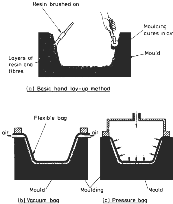
Fig. 4.67 Hand lay-up techniques
