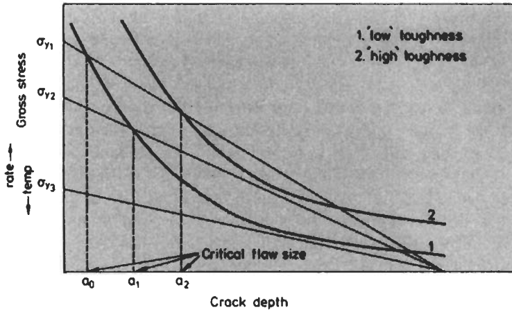
Fig. 2.69 Effect of varying stress field on flaw size for ductile/brittle transition ( K = \text{constant} )
