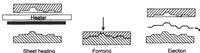
Fig. 4.53 Thermoforming between matched dies
