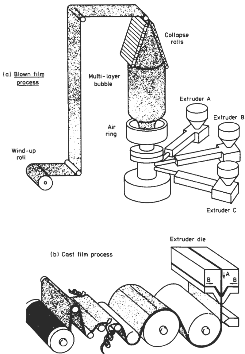
Fig. 4.28 Co-extrusion of plastic film
