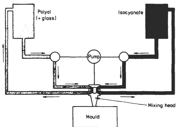
Fig. 4.47 Schematic view of reaction injection moulding
