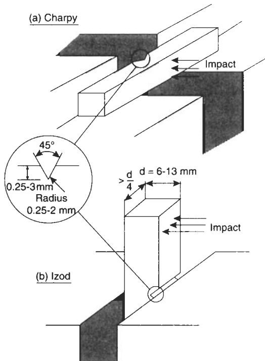
Fig. 2.81 Pendulum impact tests
