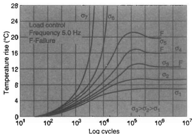
Fig. 2.73 Temperature rise during cyclic loading
