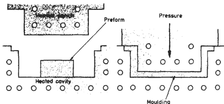
Fig. 4.62 Principle of compression moulding
