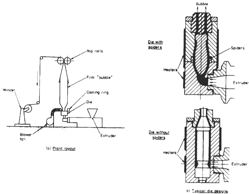
Fig. 4.20 Film blowing process
