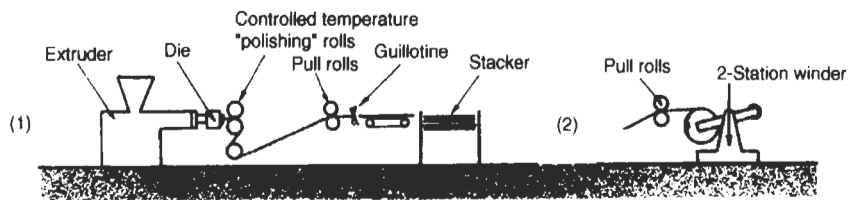
Fig. 4.19(a) Sheet extrusion (1) thick sheet (2) thin sheet
