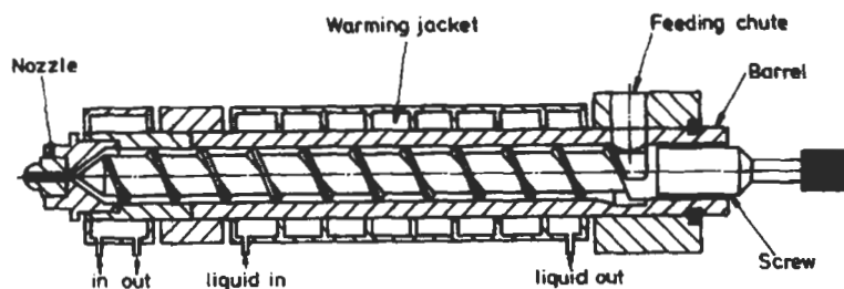
Fig. 4.50 Injection moulding of thermosets and rubbers
