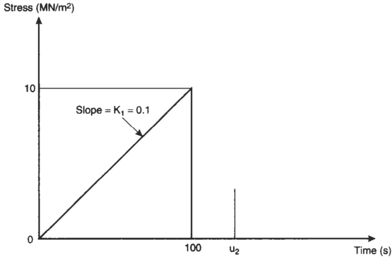
Fig. 2.48 Stress history: Example 2.15(b)
