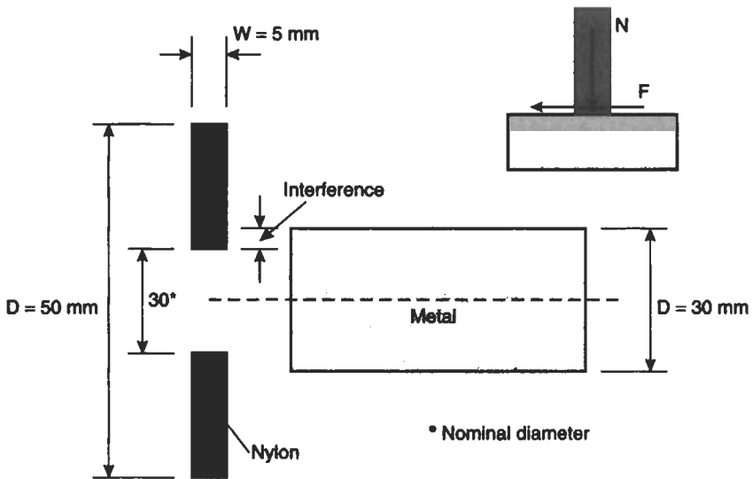
Fig. 2.17 Interference fit of nylon ring on metal shaft
