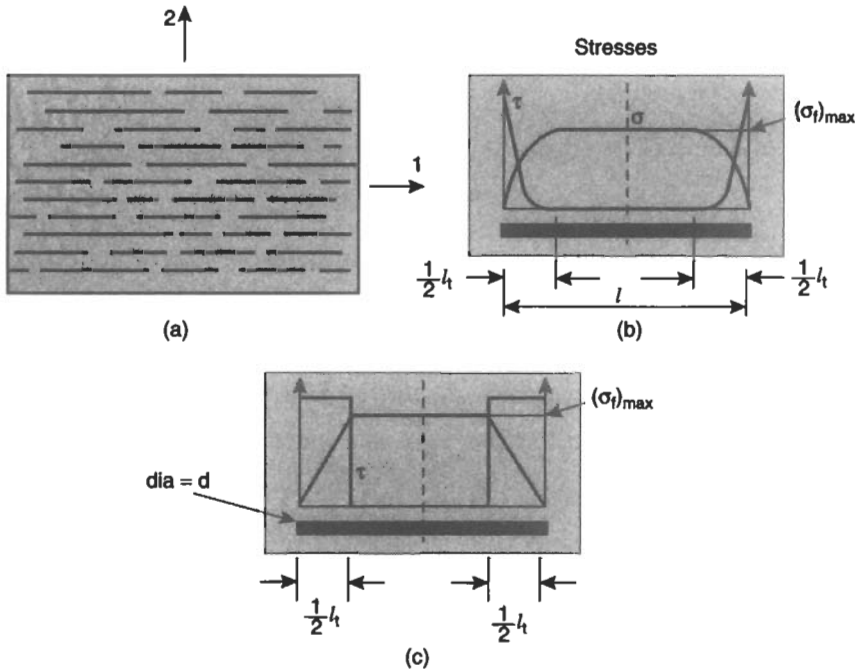
Fig. 3.29 Short Fibre Composites
