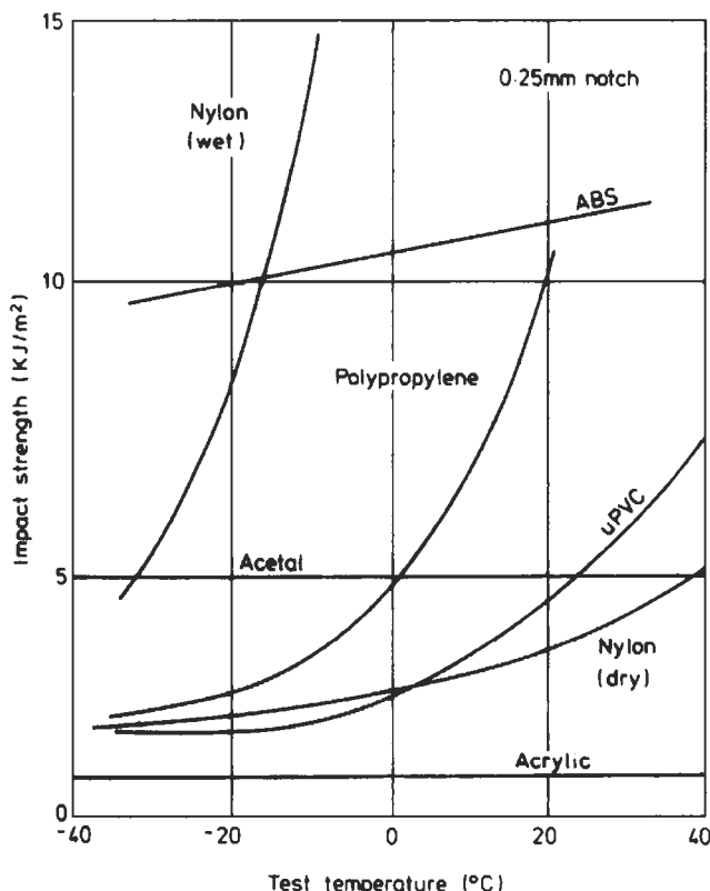
Fig. 2.80 Variation of impact strength with temperature for several thermoplastics
