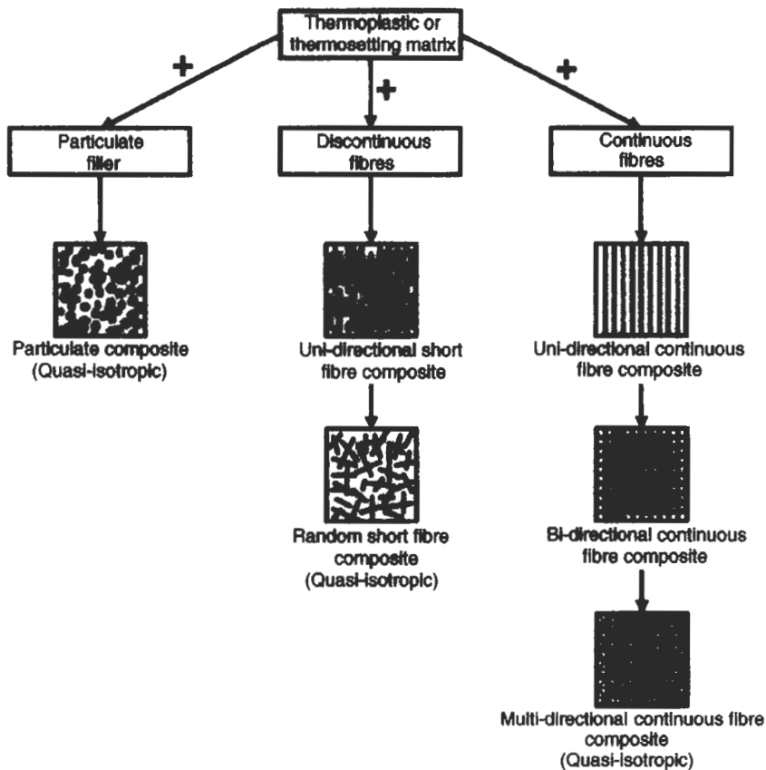
Fig. 3.1 Various types of composite (Adapted from Daniel and Ishai)
