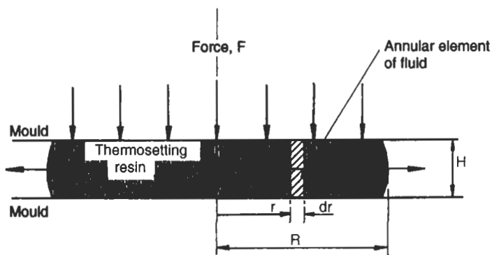
Fig. 4.63 Analysis of compression moulding
