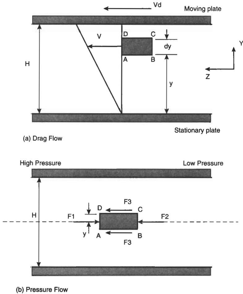
Fig. 4.7 Melt Flow between parallel plates
