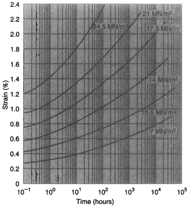
Fig. 2.51 Creep curves for acetal
