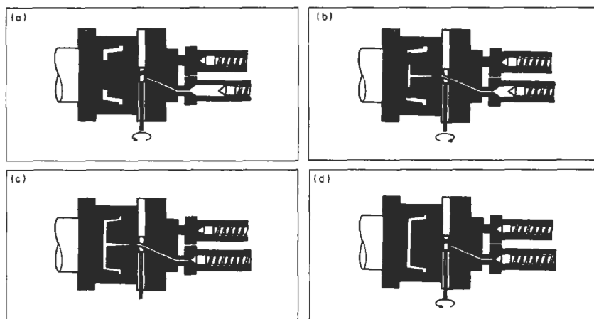
Fig. 4.44 Stages in sandwich moulding process
