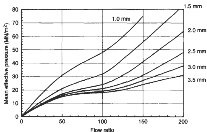
Fig. 4.42 Clamping pressures for different cavity geometries (typical values for easy flow materials)
