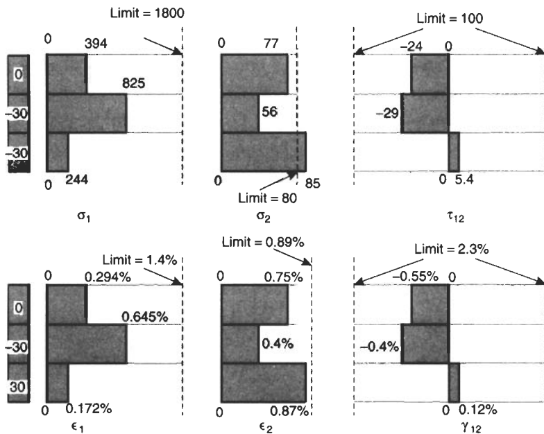
Fig. 3.31 Stress and strain in the plies, Example 3.21
