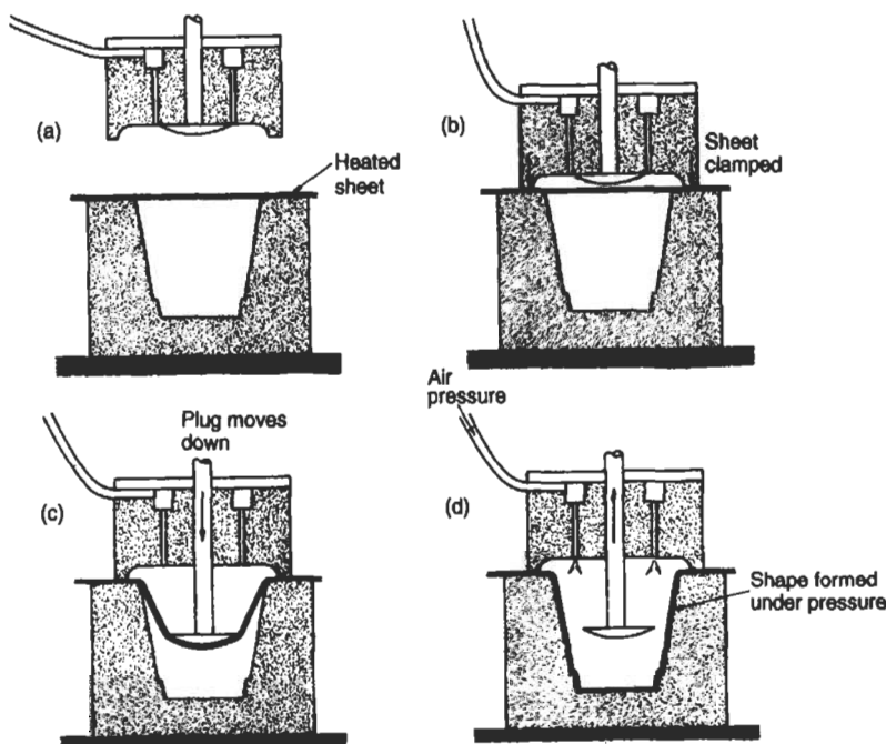
Fig. 4.52 Pressure forming process
