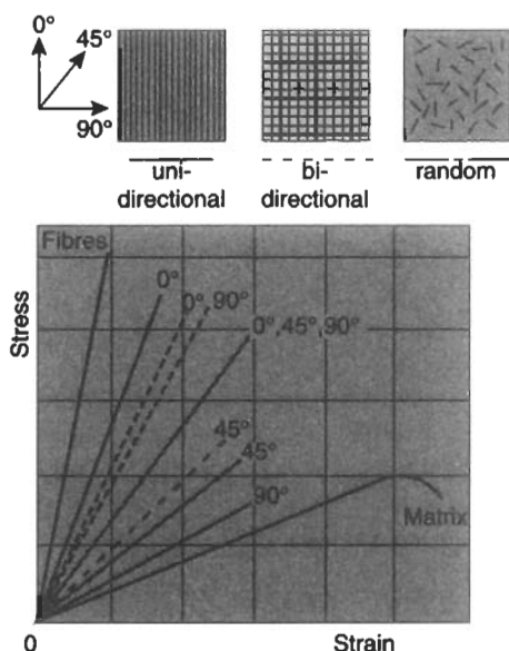
Fig. 3.4 Stress-strain behaviour for several types of fibre reinforcement
