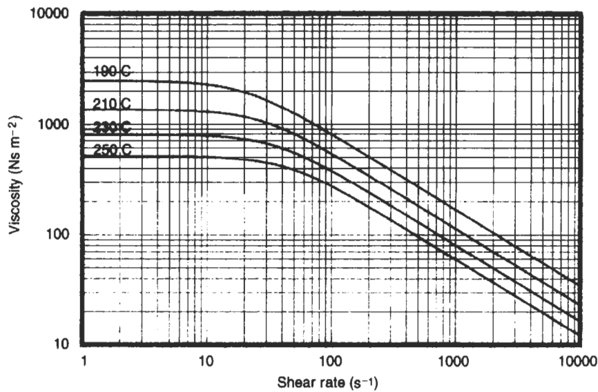
Fig. 5.2 Viscosity curves for polypropylene
