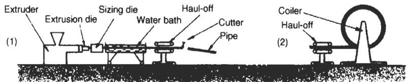
Fig. 4.19(b) Pipe extrusion (1) rigid pipe (2) flexible pipe
