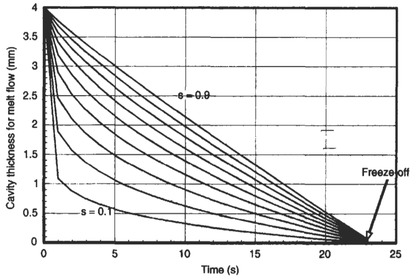
Fig. 5.26 Variation of Cavity Depth with Time
