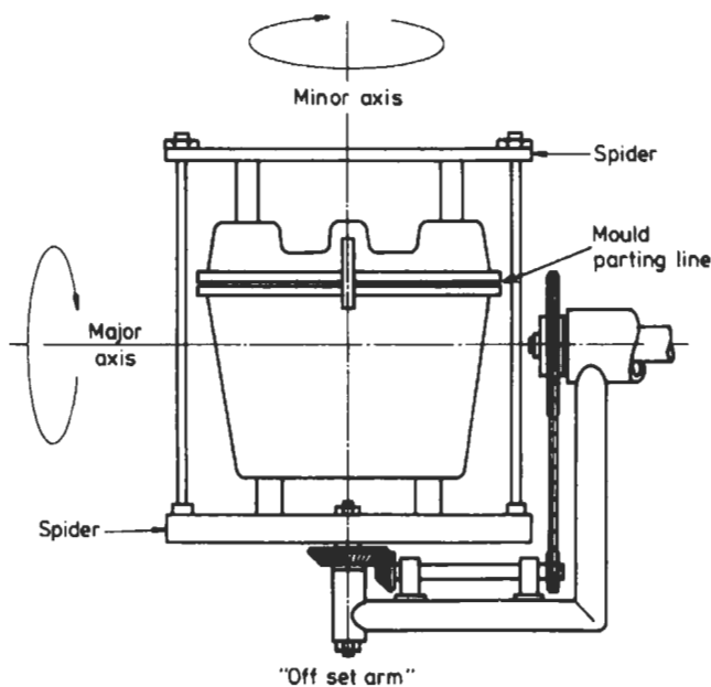
Fig. 4.60 Typical 'off-set arm' rotation
