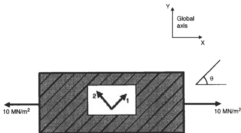
Fig. 3.12 Unidirectional Kevlar/epoxy composite (single ply)
