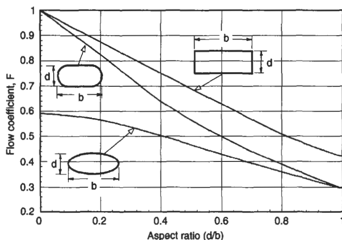
Fig. 4.13 Flow coefficient as a function of channel geometry
