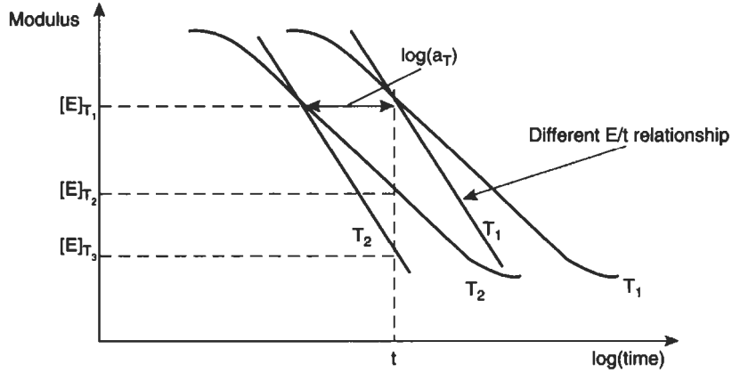
Fig. 2.60 Various modulus–time curves
