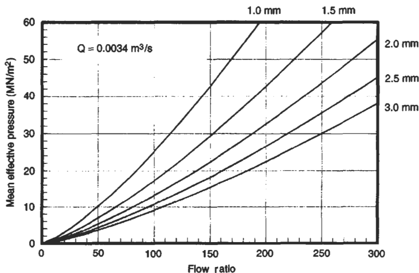
Fig. 5.27 Variation of Cavity Pressure with Flow Ratio
