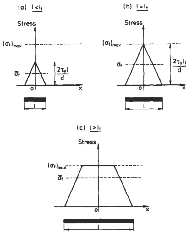
Fig. 3.30 Stress variations in short fibres
