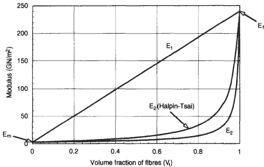
Fig. 3.7 Variation of longitudinal and transverse modulus in unidirectional composites
