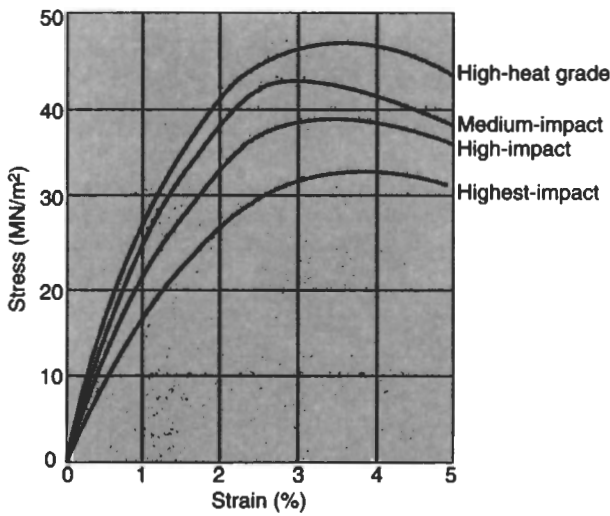
Fig. 1.5 Effect of grade on mechanical properties of ABS
