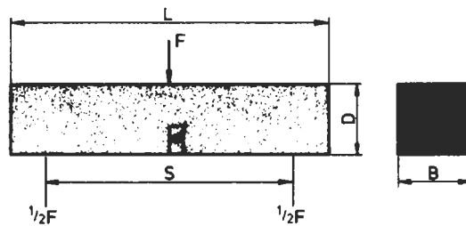
Fig. 2.83 Charpy test piece
