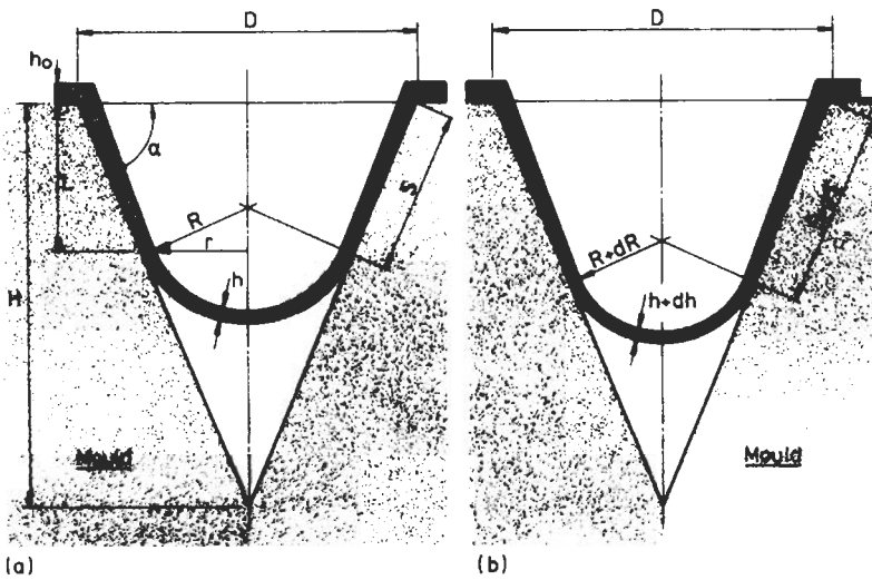
Fig. 4.55 Analysis of thermo forming
