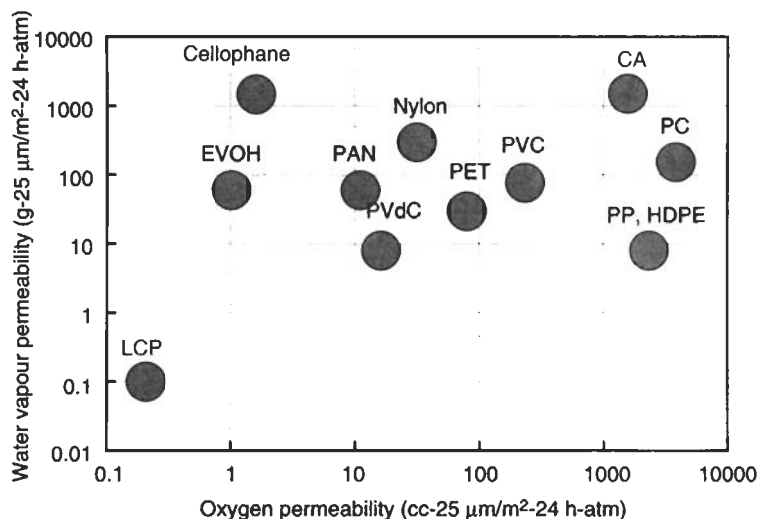
Fig. 1.13 Permeability data for a range of plastics
