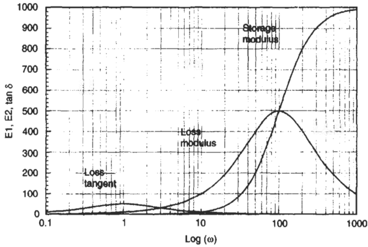
Fig. 2.55 Typical variation of E_1 , E_2 and loss tangent for a viscoelastic material
