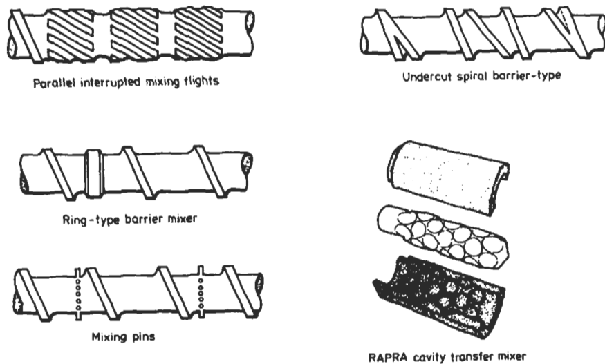
Fig. 4.4 Typical designs of mixing zones
