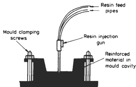
Fig. 4.74 Resin injection process
