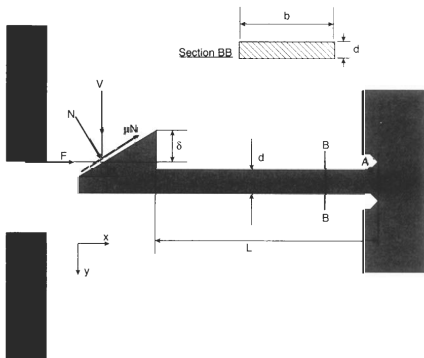
Fig. 2.22 Snap fit for Example 2.10
