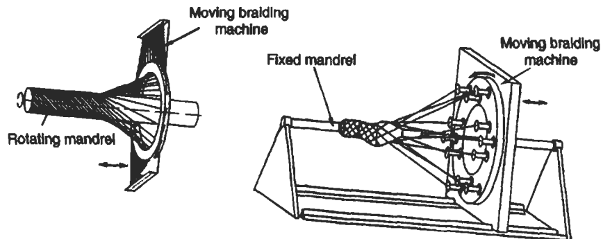
Fig. 4.76 Two types of filament winding
