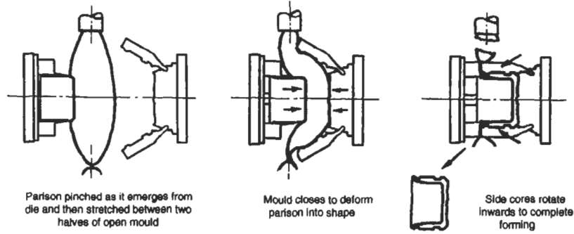
Fig. 4.22 Stages in blow moulding of complex hollow container
