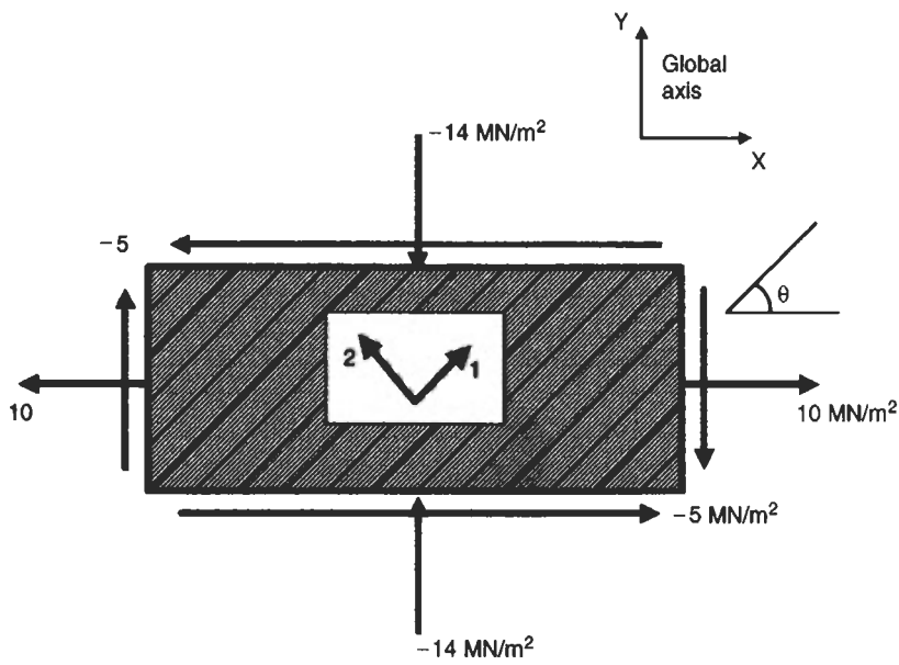
Fig. 3.14 Unidirectional carbon fibre single ply composite
