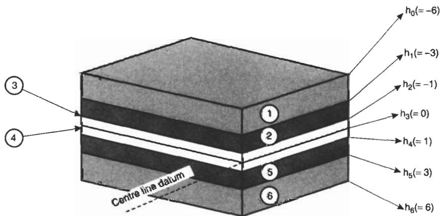
Fig. 3.21 Six ply laminate
