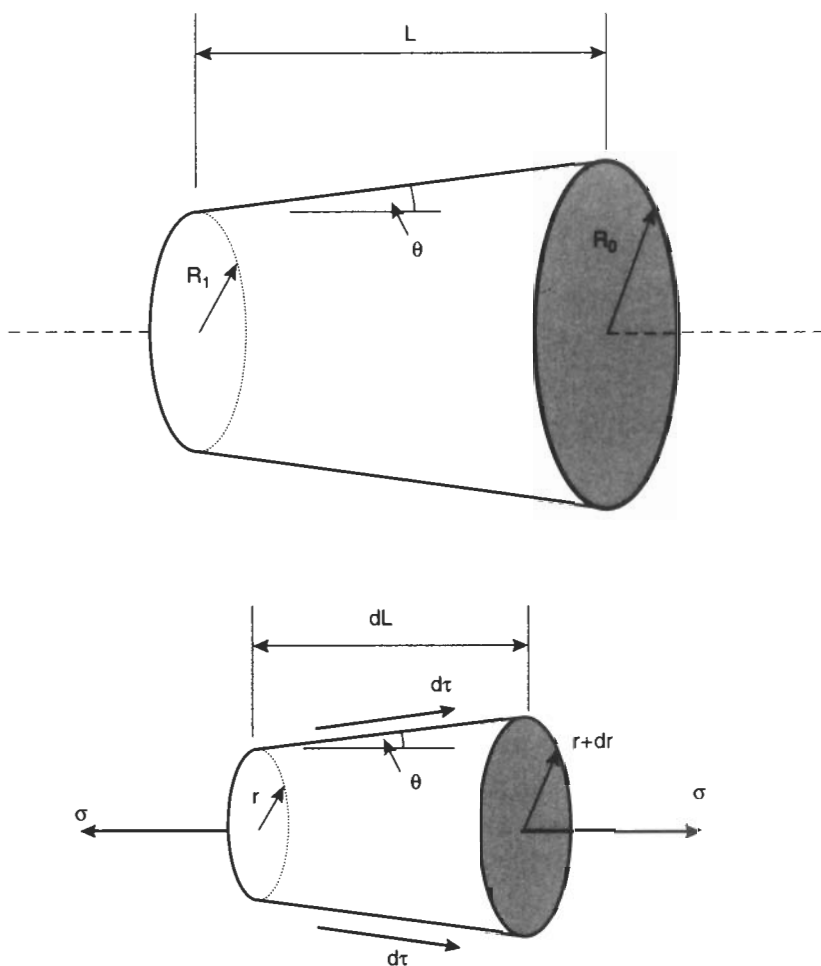
Fig. 5.8 Analysis of Coni-Cylindrical Die
