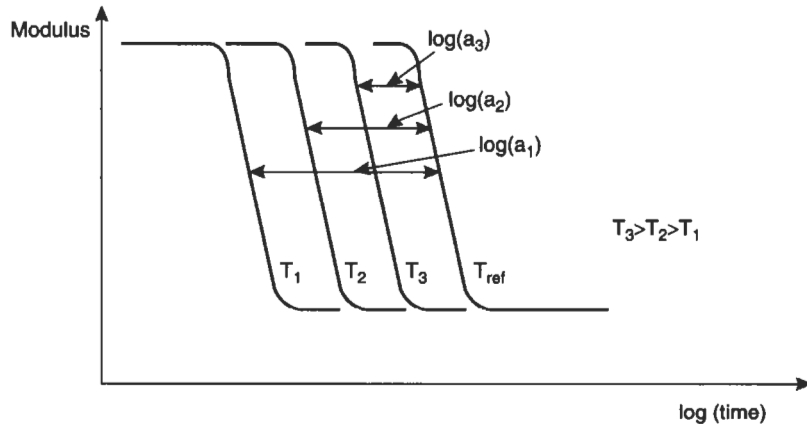
Fig. 2.58 Modulus–time curves for a range of temperatures
