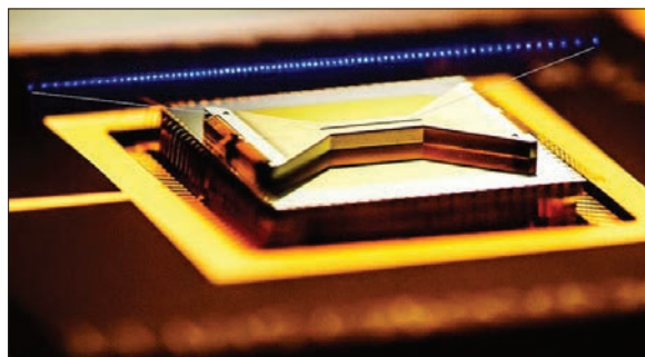
Quantum business Montage of a photo of the chip containing the trapped ions and an image of the ions in a 1D array.
