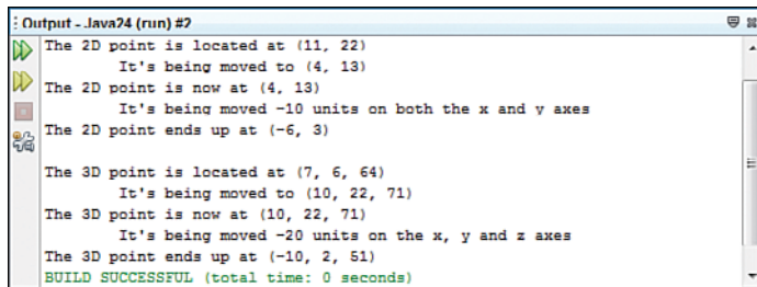
FIGURE 12.3 The output of the PointTester program.
