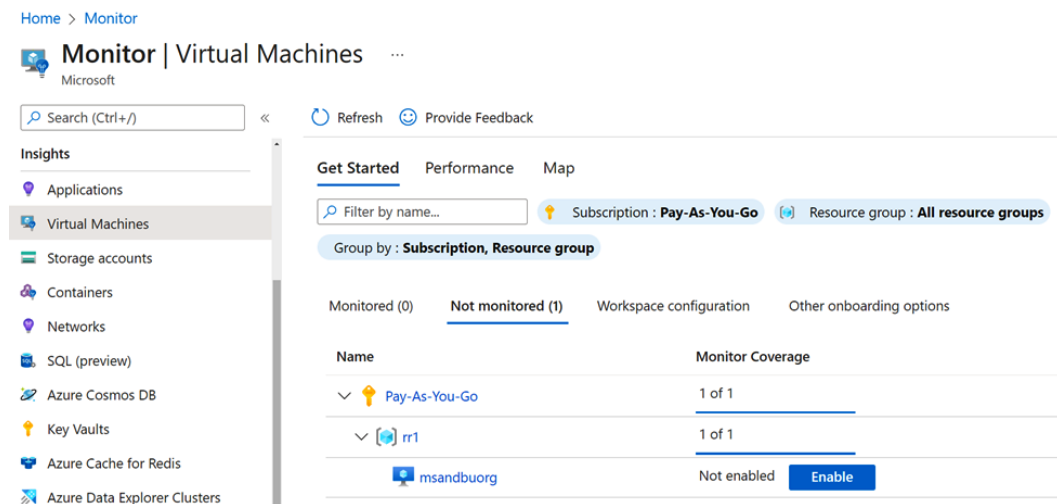
Figure 3.5 – Enabling logging from a VM in Azure
