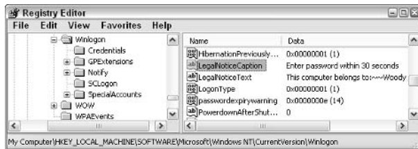
• Figure 8-7: Final settings for the Winlogon Registry key.
