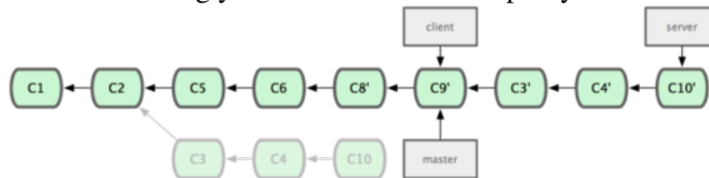
Figure 3.34: Rebasing your server branch on top of your master branch
