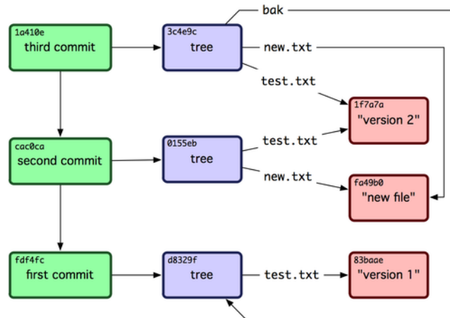
Figure 9.3: All the objects in your Git directory
