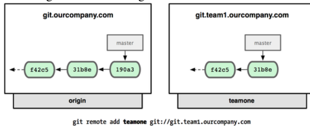
Figure 3.25: Adding another server as a remote
