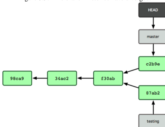
Figure 3.9: The branch histories have diverged.
