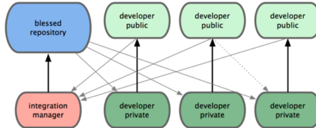
Figure 5.2: Integration-manager workflow
