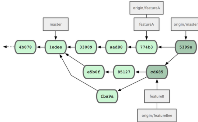
Figure 5.14: Jessica’s history after merging both her topic branches
