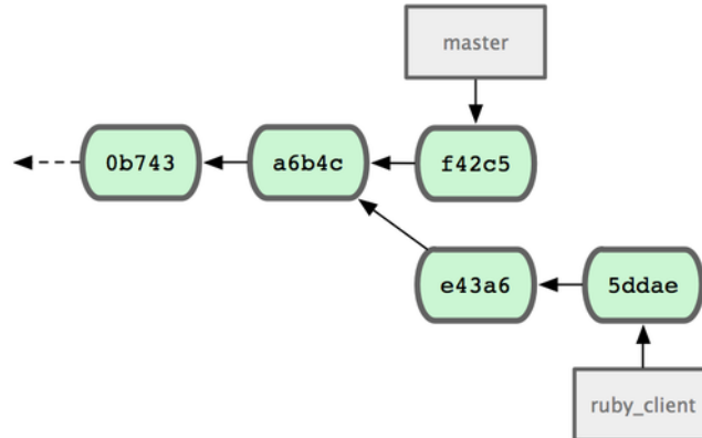
Figure 5.26: Example history before a cherry pick
