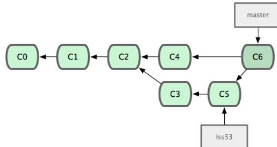
Figure 3.17: Git automatically creates a new commit object that contains the merged work.
