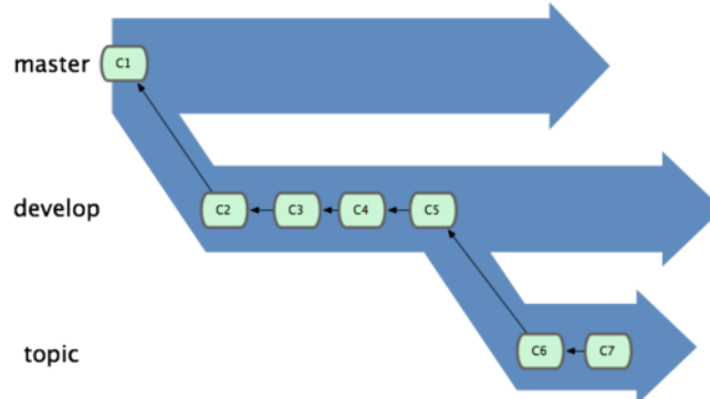
Figure 3.19: It may be helpful to think of your branches as silos.
