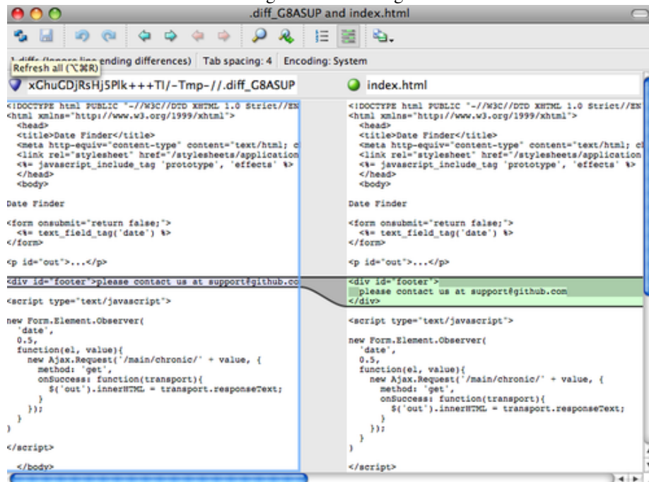
Figure 7.1: P4Merge
