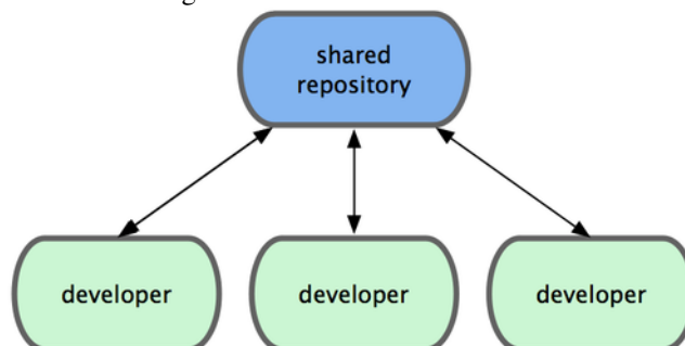
Figure 5.1: Centralized workflow
