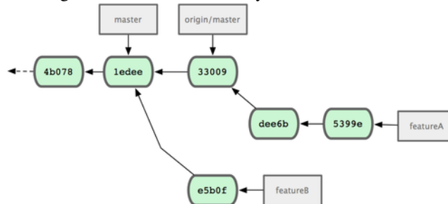
Figure 5.17: Commit history after featureA work
