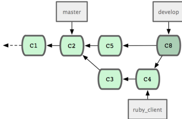
Figure 5.22: After a topic branch merge
