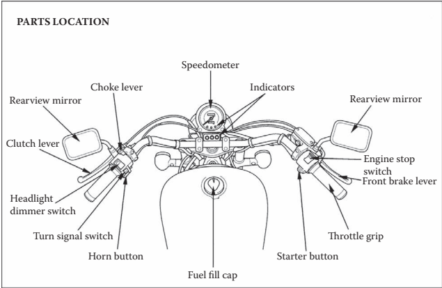
FIGURE 5.18 Illustration using words to call out part names. Using words and arrows to call out parts makes it quicker for the user to find the part name, but limits the amount of information that can be shown in one drawing and requires an extra step for translation. Source: From Honda Owner's Manual 97VT1100C2 Shadow 1100 , American Honda Motor Company, Torrance, CA, 1996, p. 11, © Copyright by American Honda Motor Co., Inc. With permission.
