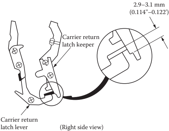
FIGURE 7.2 Example of a graphic that conveys information about tolerances. Note the effective use of a close-up to avoid cluttering the drawing and to make it more readable. Source: From Single-Element Typewriter, Model 200, Service Manual , Silver Reed America, Inc., Torrance, CA, p. 45. With permission.
