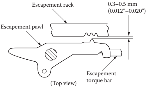
FIGURE 7.1 Example of a graphic used to convey specifications and tolerances. Source: From Single-Element Typewriter, Model 200, Service Manual , Silver Reed America, Inc., Torrance, CA, p. 44. With permission.
