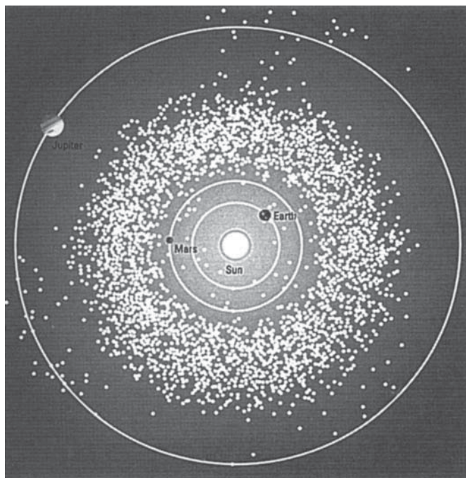
Figure 2: The solar system showing the location of the asteroid belt between Mars and Jupiter which, though the details vary, many ancient and modern accounts suggest is the remains of a planet or part of a planet.
